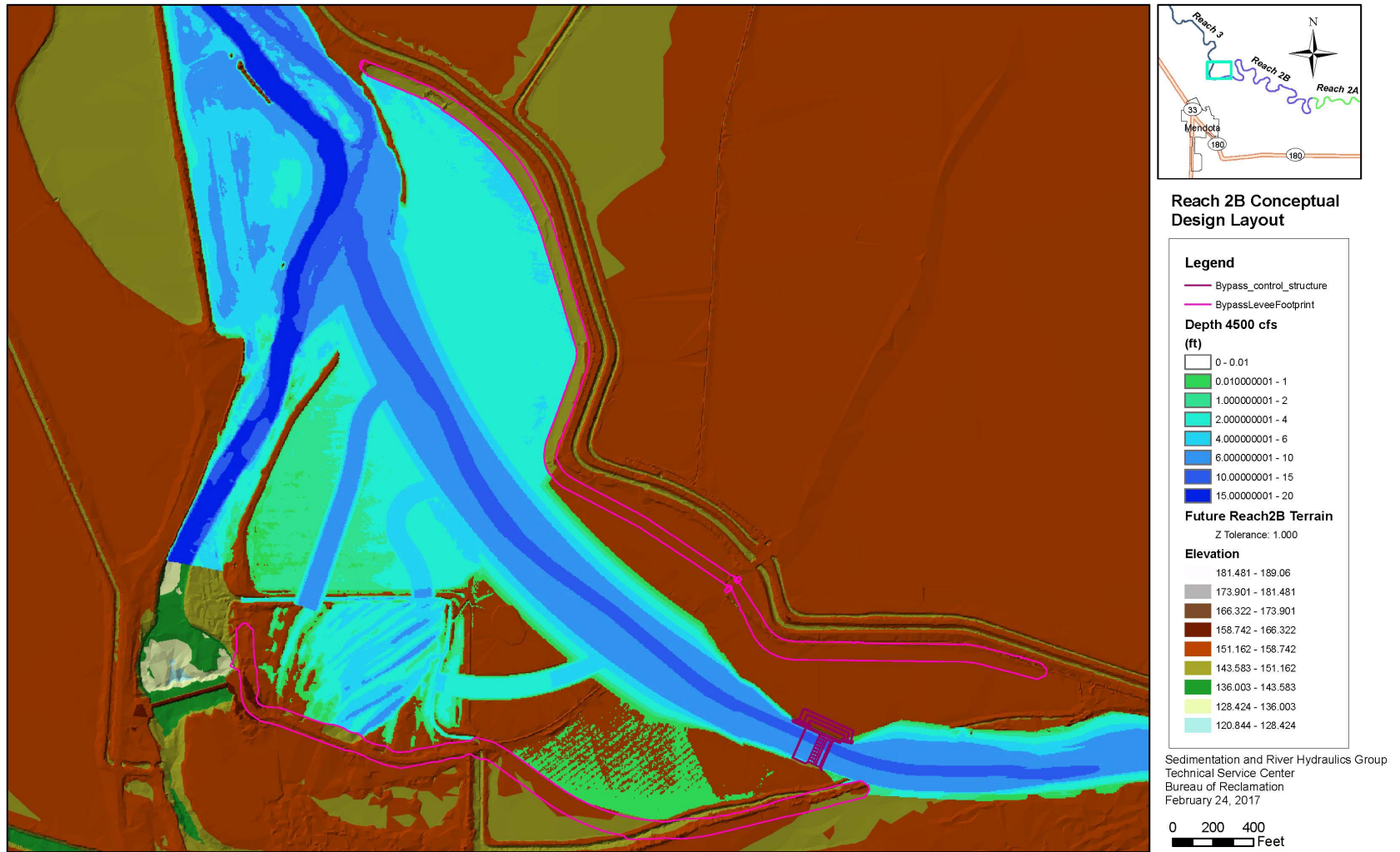
Figure 5-14.—Simulated depth distribution in the Bypass using SRH-2D at a flow of 4,500 cfs in Bypass.
