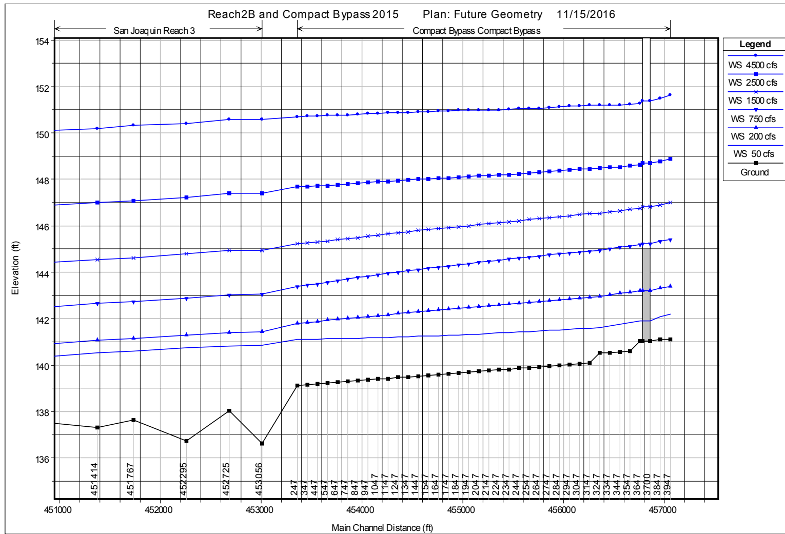
Figure 5-4.—Water surface profiles in Bypass for flows between 100 and 4,500 cfs for expected future conditions after channel adjustment.
