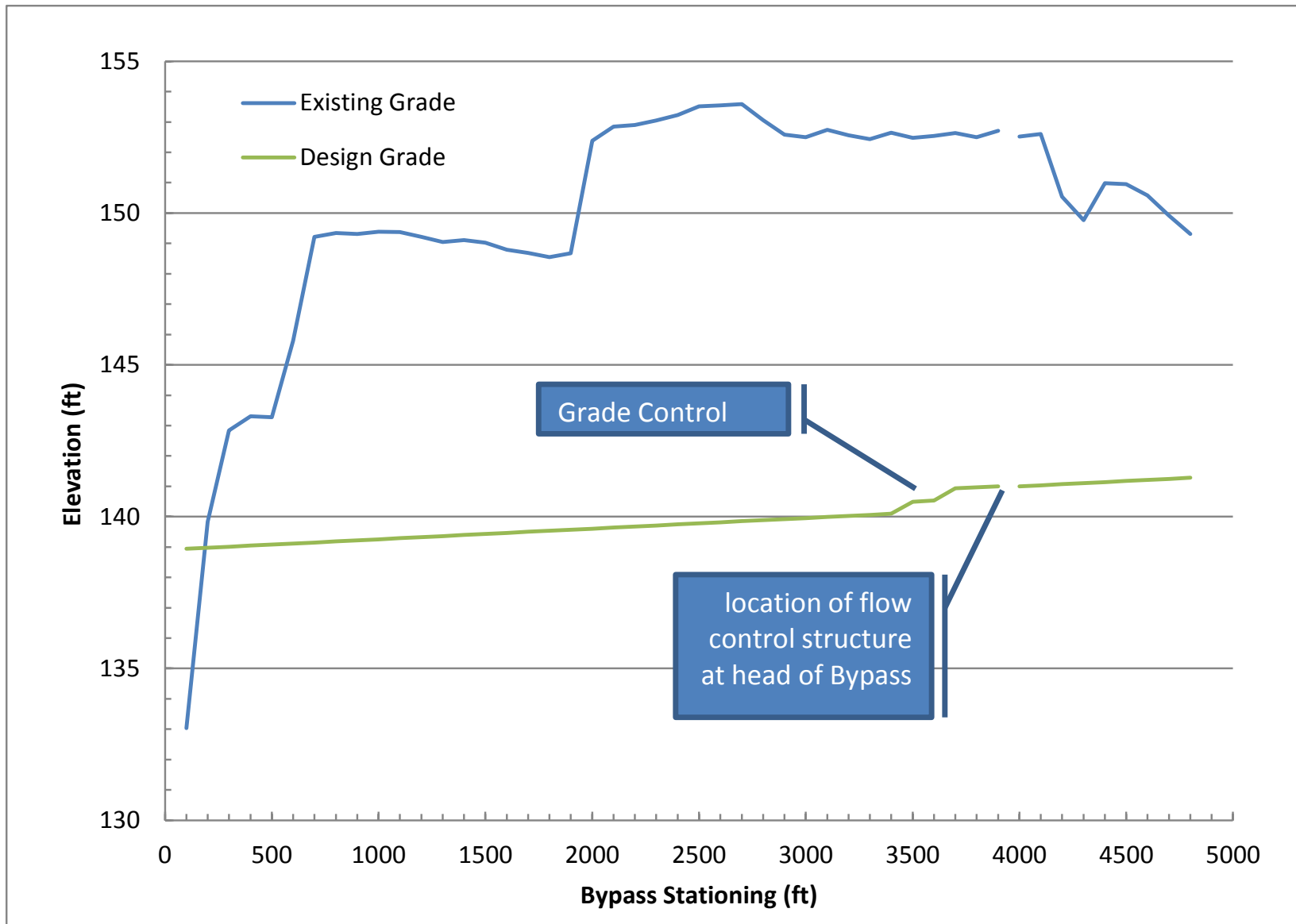
Figure 4-2.—Existing Grade and Design Grade along the Bypass centerline.
