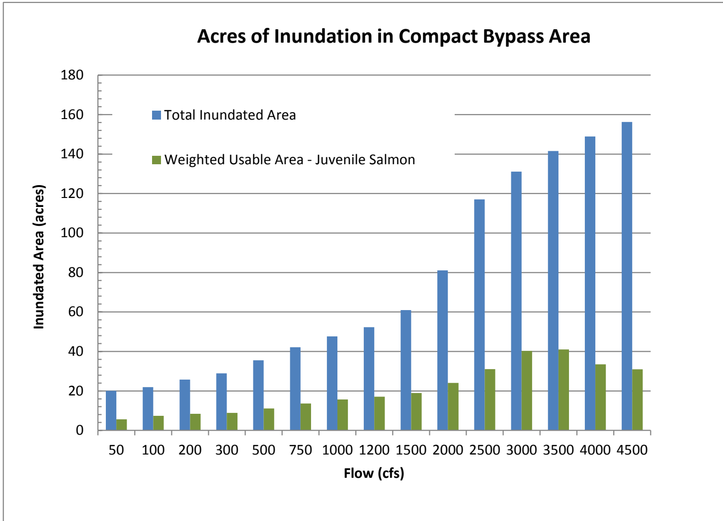
Figure 5-19.—Inundated area from SRH-2D simulated area for a range of flows.
