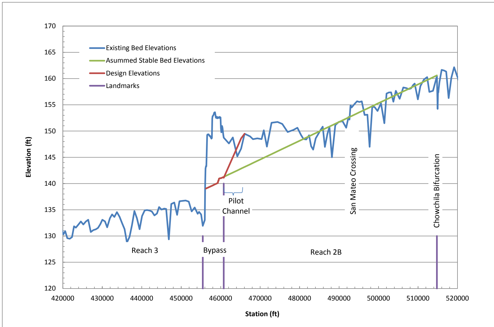
Figure 4-1.—Existing and design profiles in Reach 2B through Compact Bypass.
