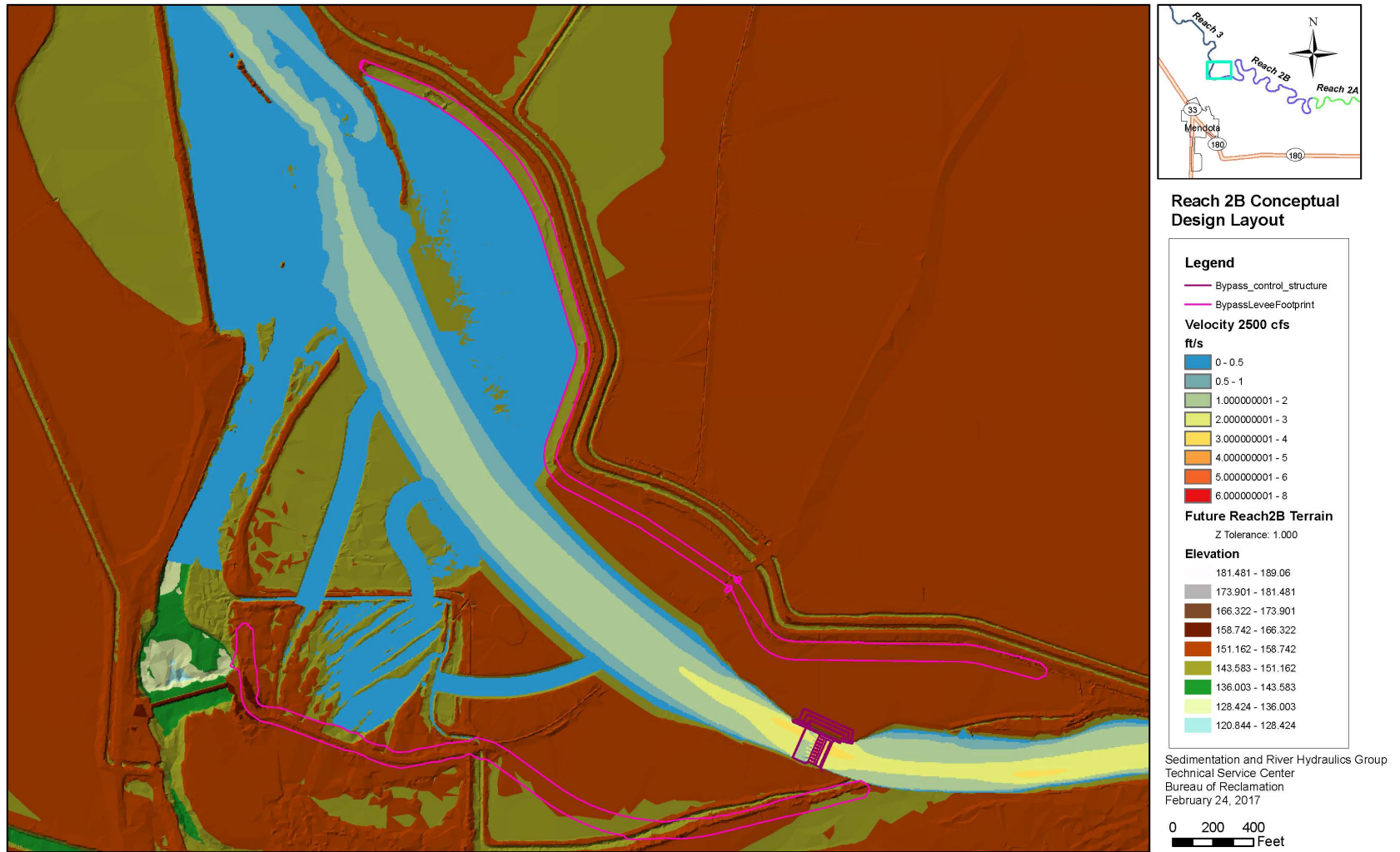
Figure 5-16.—Simulated velocity distribution in the Bypass using SRH-2D at a flow of 2,500 cfs in Bypass.
