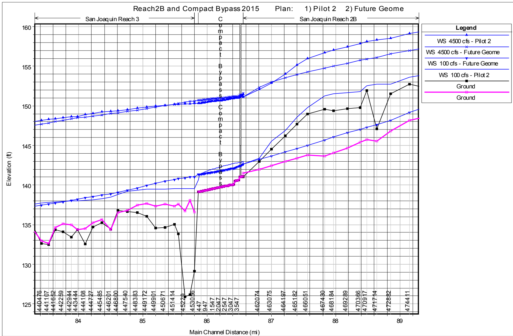
Figure 5-5.—Water surface profiles in Bypass for flows of 100 and 4,500 cfs for conditions immediately after construction of Bypass and then expected future conditions after channel adjustment.
