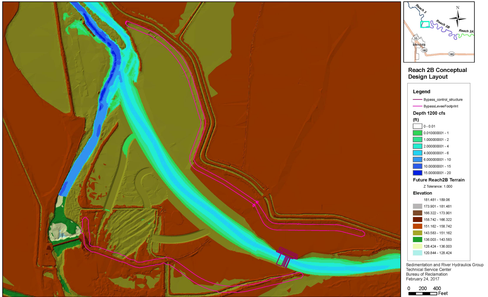
Figure 5-12.—Simulated depth distribution in the Bypass using SRH-2D at a flow of 1,200 cfs in Bypass.
