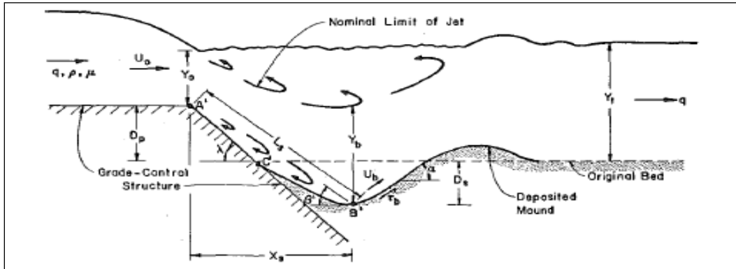
Figure 4-5.—Scour downstream of grade control, figure from Borman and Julien (1991).
