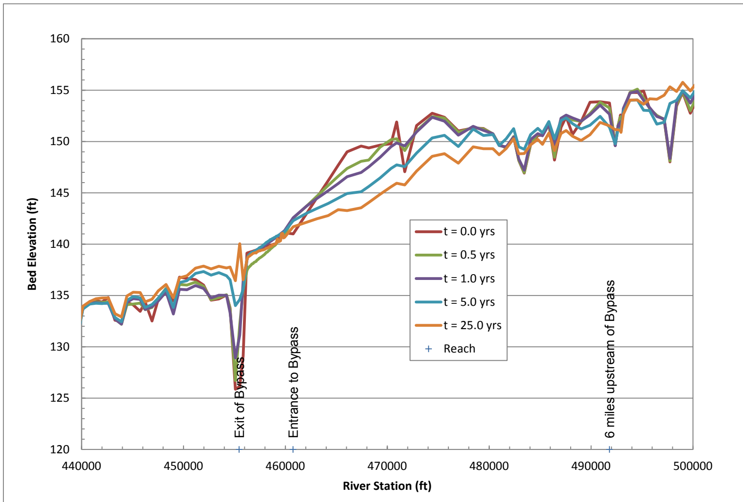
Figure 5-21.—Evolution of Reach 2B and 3 bed profile with pilot channel.
