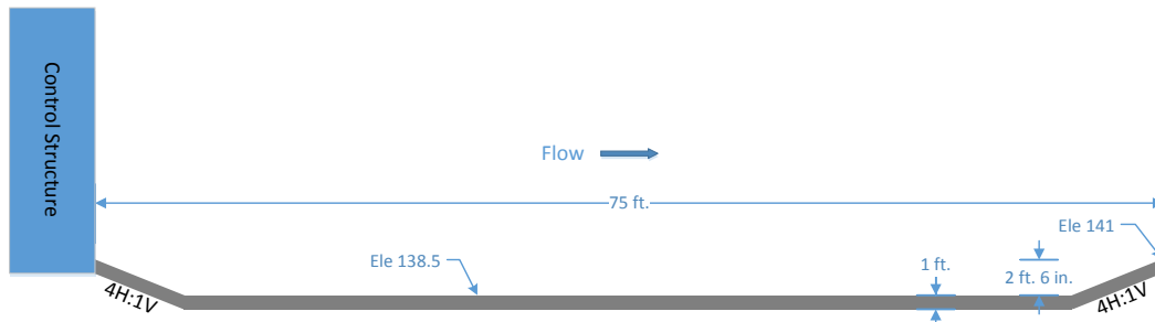
Figure 4-4.—Conceptual drawing of stilling basin downstream of Compact Bypass Control Structure.
