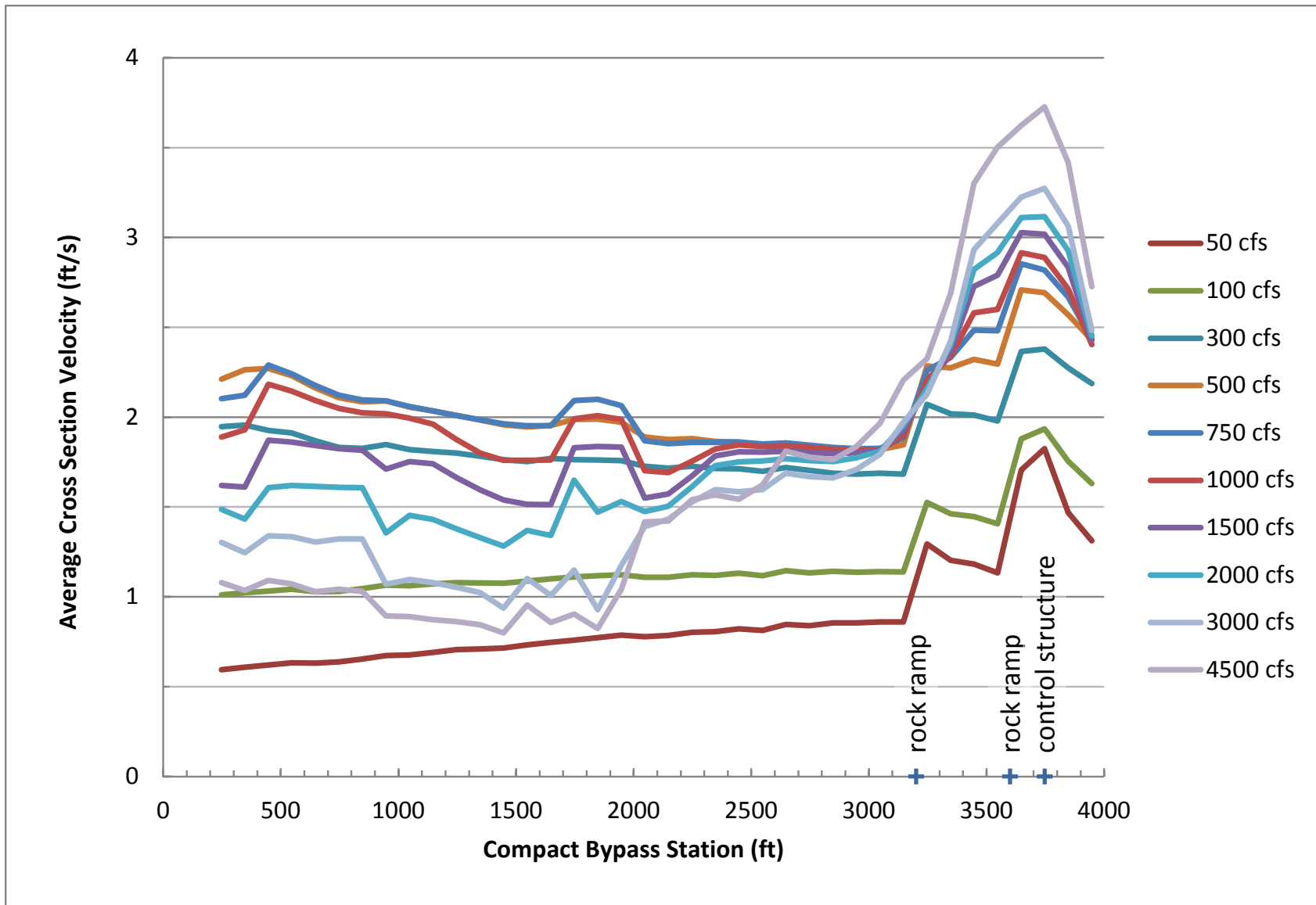
Figure 5-9.—Average cross section velocity in Bypass for flows between 50 and 4,500 cfs.
