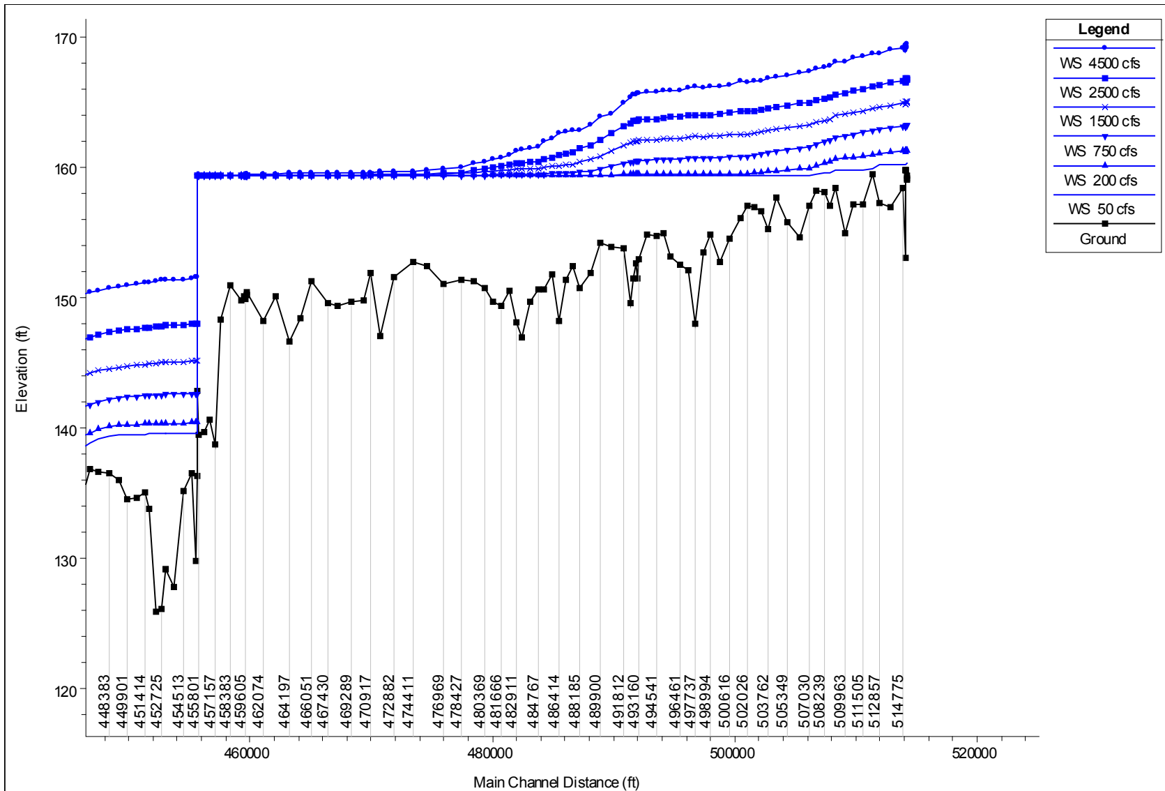
Figure 5-20.—Water surface profiles used for levee design in Reach 2B for Delivery Conditions assuming that the water surface required for delivery rises 5 ft relative to ground surface to account for subsidence.
