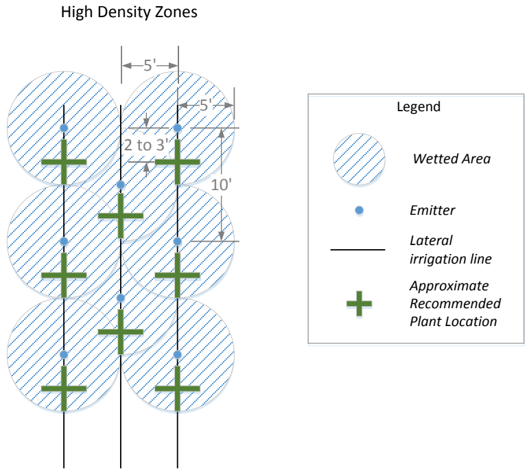
Figure 4-14.— Irrigation and Emitter spacing for High Density Irrigation Zone.
