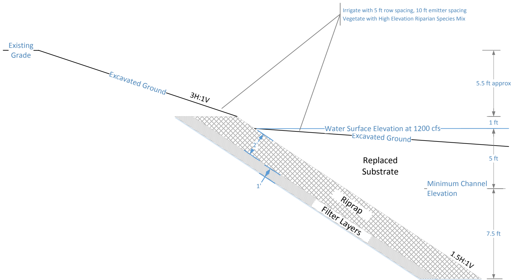
Figure 4-7.—Conceptual cross section of riprap lined bank.
