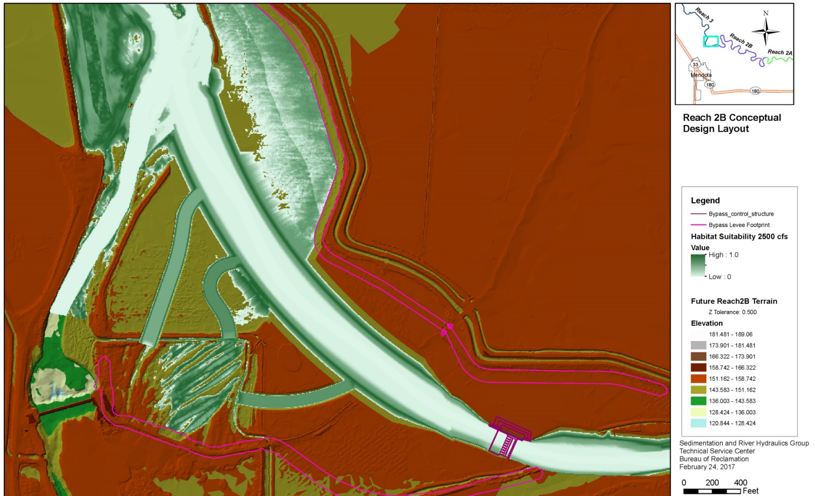
Figure 5-18.—Simulated Habitat Suitability Index distribution in the Bypass using SRH-2D at a flow of 2,500 cfs in Bypass.
