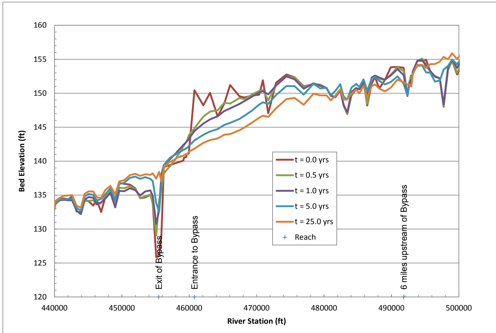
Figure 5-23.—Evolution of Reach 2B and 3 bed profile without pilot channel.
