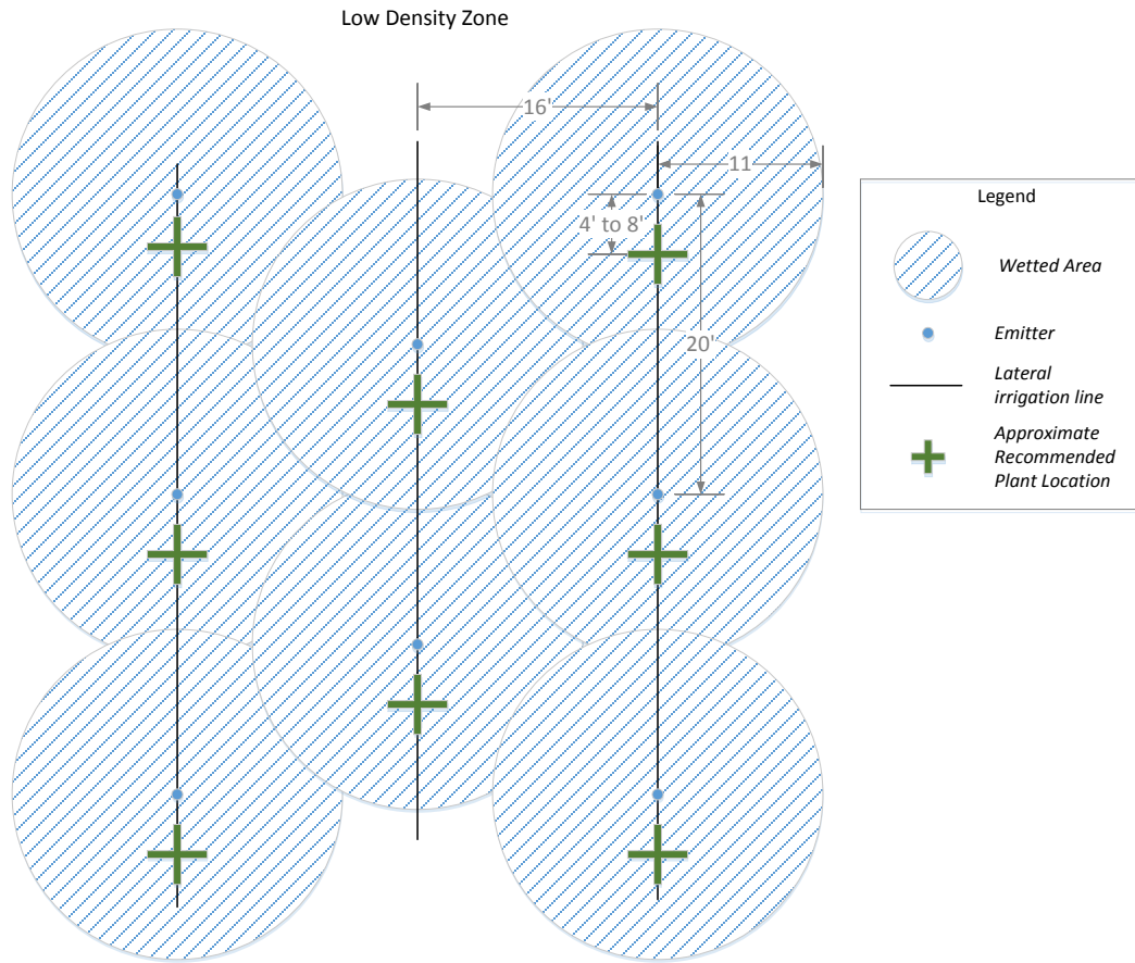
Figure 4-16.— Irrigation and Emitter spacing for Low Density Irrigation Zone.
