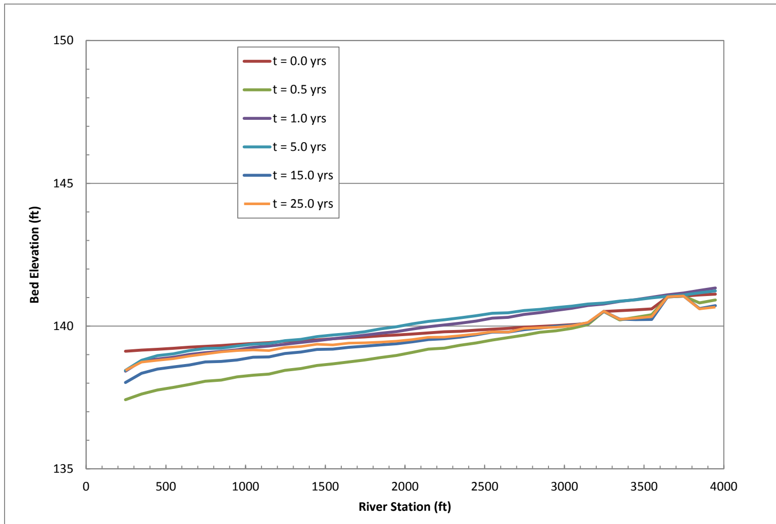
Figure 5-22.—Evolution of Compact Bypass bed profile with pilot channel. River station is relative to downstream end of Compact Bypass Channel.
