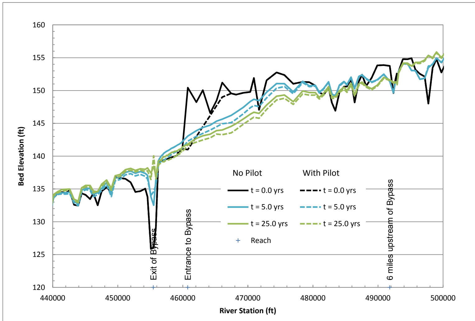
Figure 5-26.— Comparison of bed elevation with and without pilot channel for initial conditions, 5 years, and 25 years after beginning simulation.
