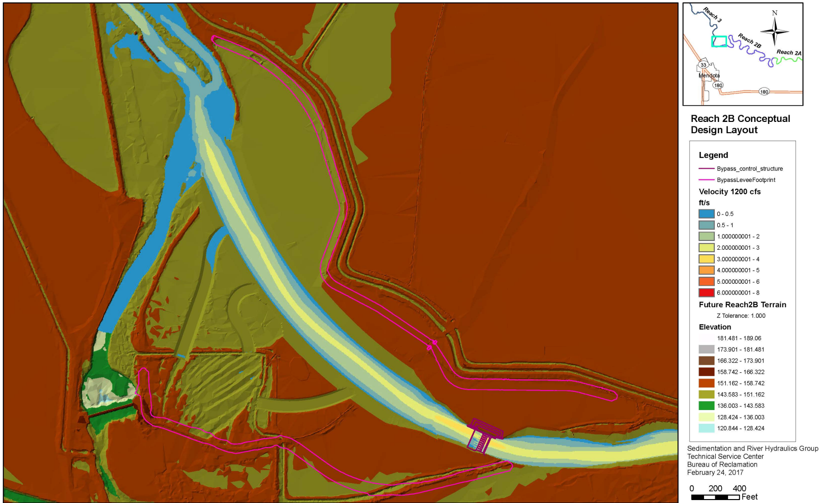
Figure 5-15.—Simulated velocity distribution in the Bypass using SRH-2D at a flow of 1,200 cfs in Bypass.
