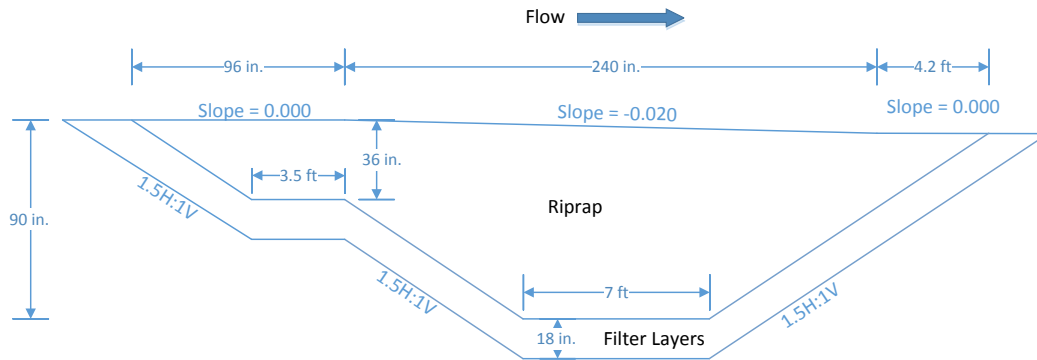
Figure 4-6.— Conceptual profile section of grade control structure.
