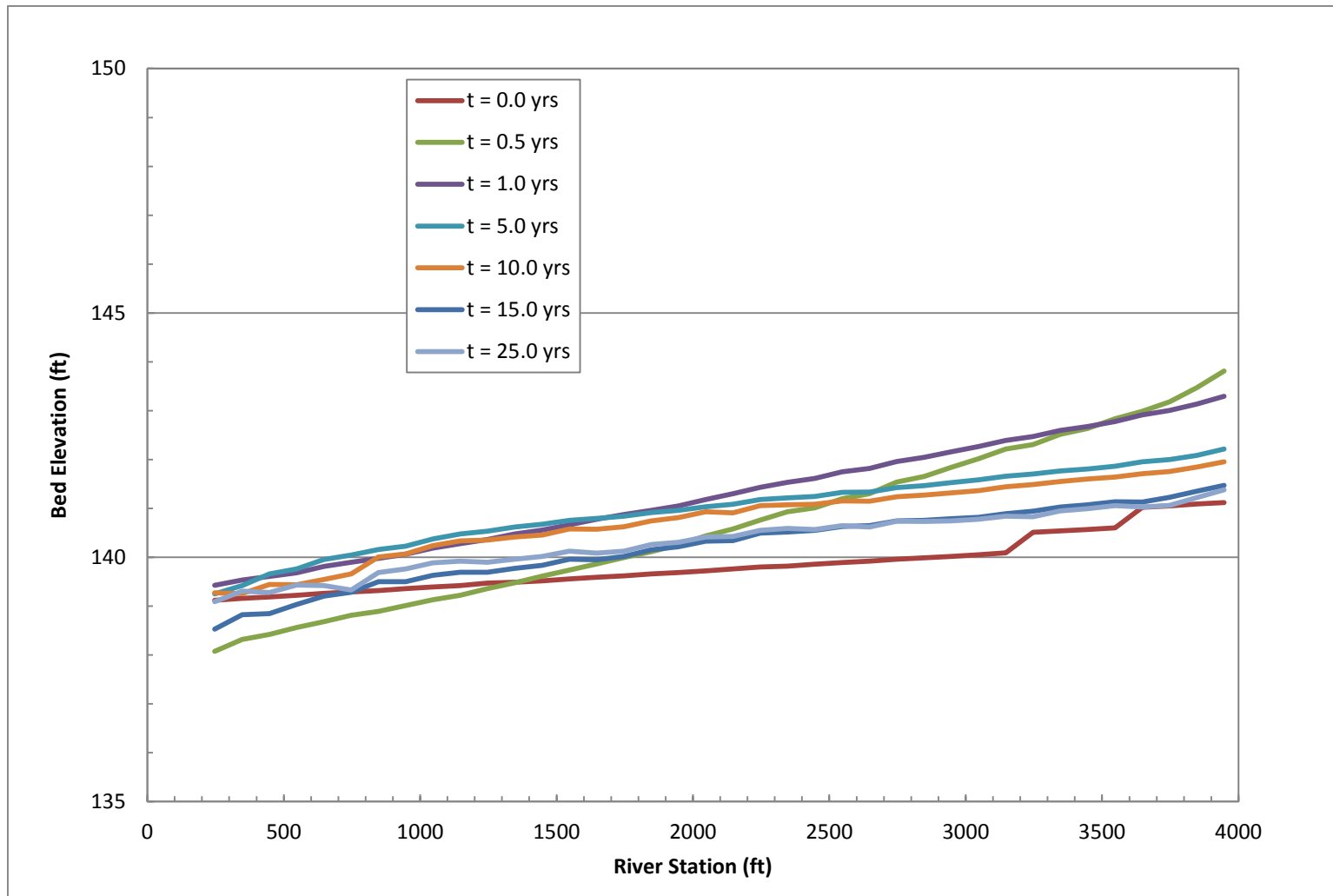
Figure 5-24.—Evolution of Compact Bypass bed profile without pilot channel. River station is relative to downstream end of Compact Bypass Channel.
