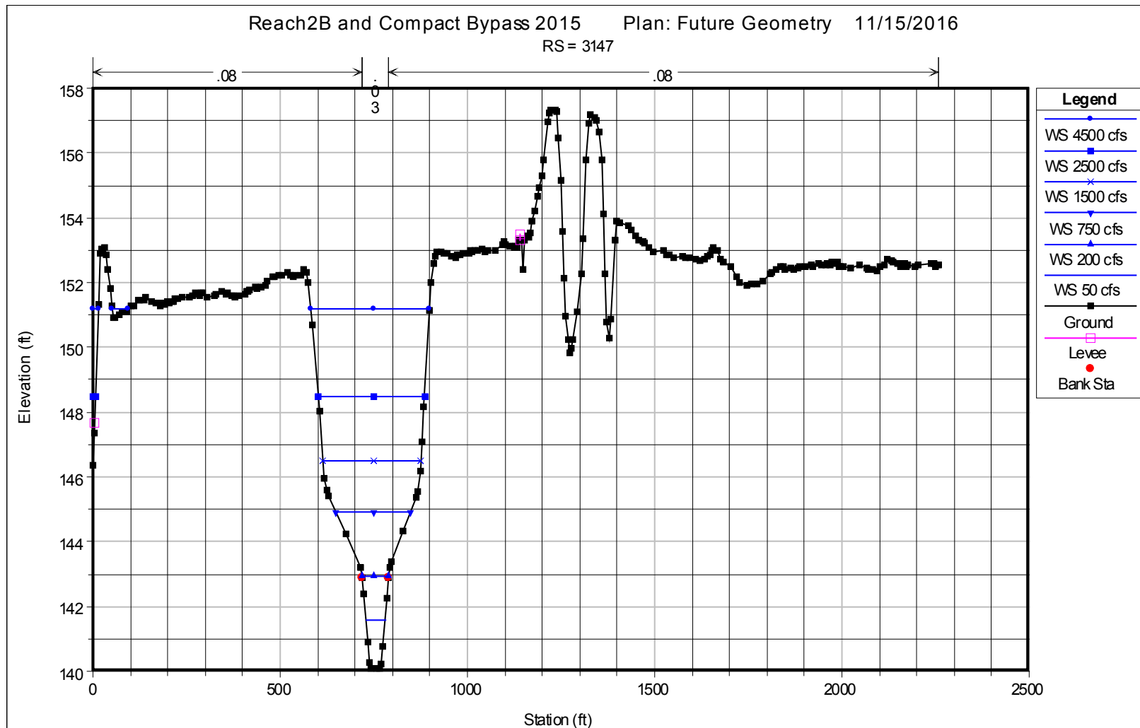
Figure 5-6.—Cross section 3147 in Bypass showing water surfaces.
