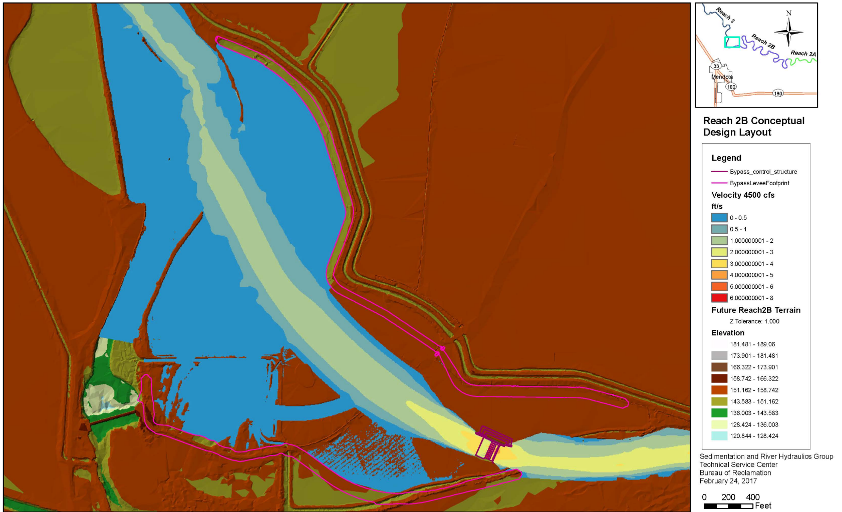
Figure 5-17.—Simulated velocity distribution in the Bypass using SRH-2D at a flow of 4,500 cfs in Bypass.
