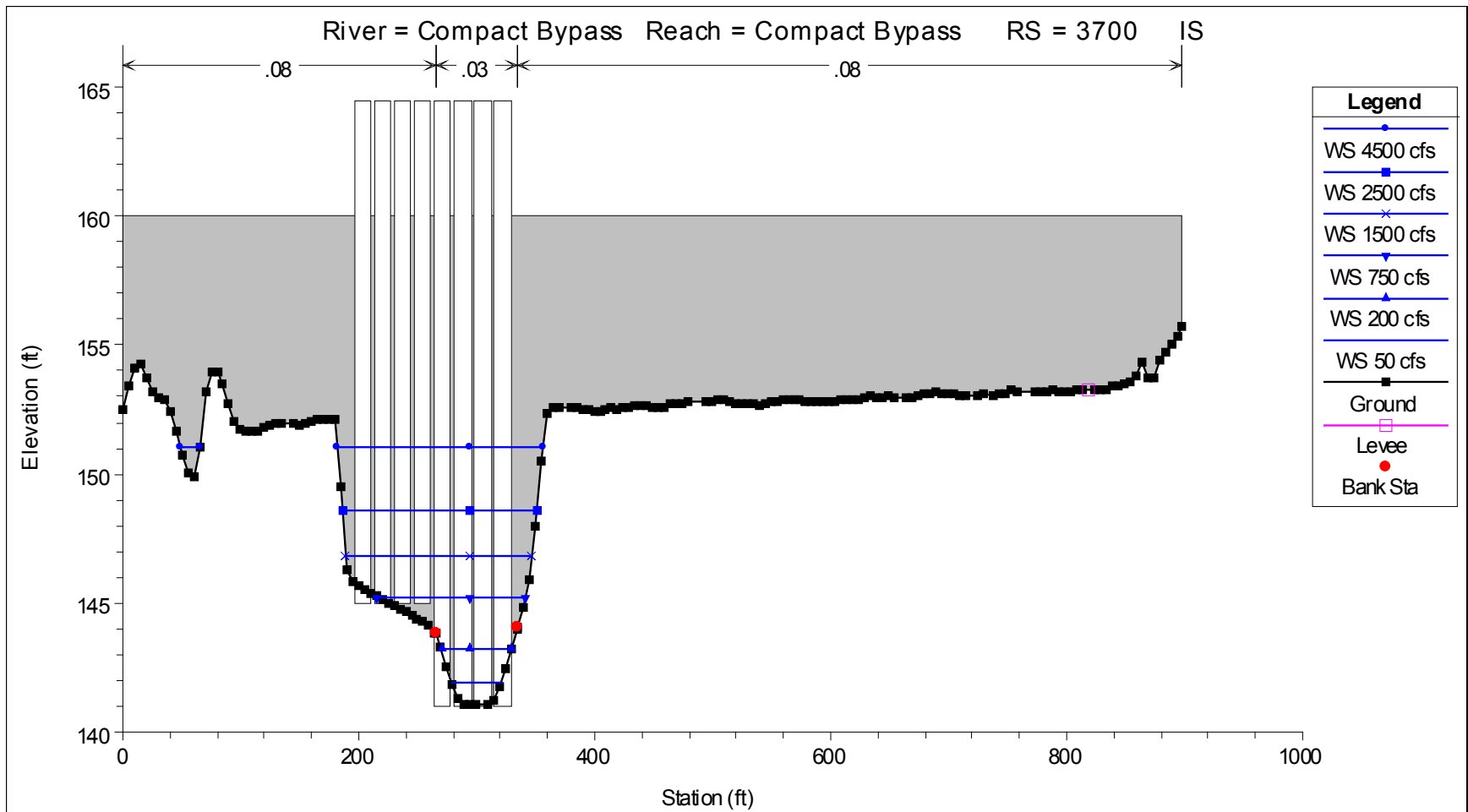
Figure 5-11.—Water surfaces at control structure at head of the Bypass with all gates open. The structure walls and abutments are shown in gray.
