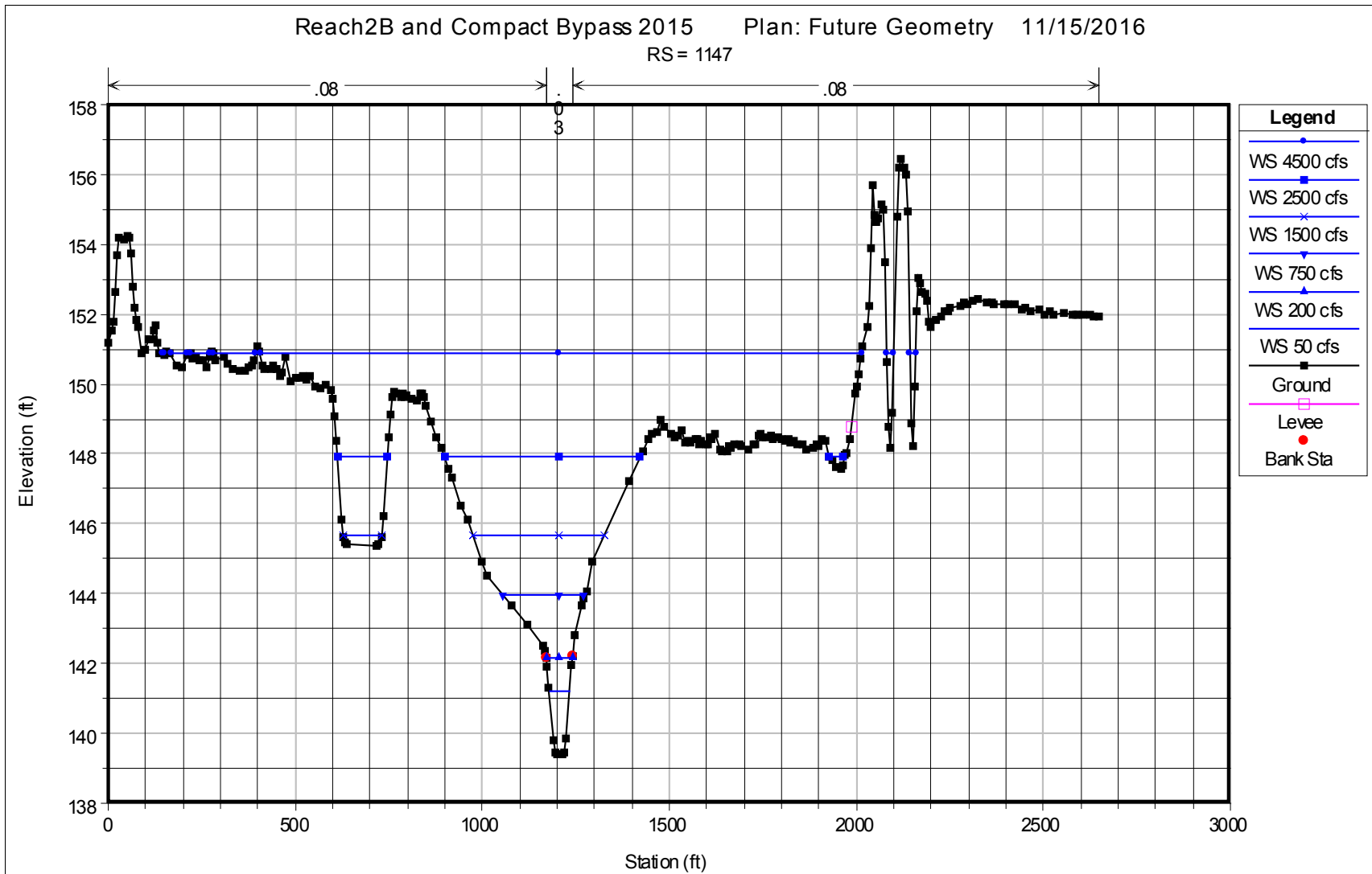
Figure 5-8.—Cross section 1147 in Bypass showing water surfaces.
