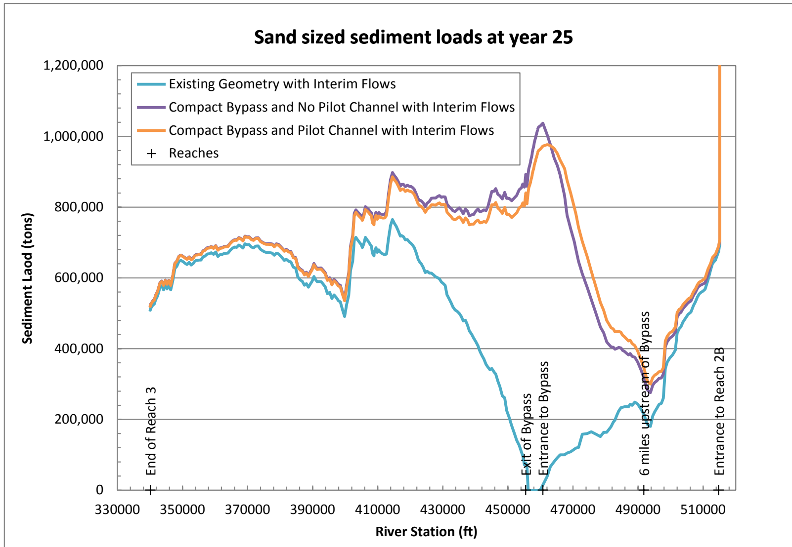
Figure 5-27.— Comparison of sand sized cumulative sediment load in simulated reach at year 25 for Existing Conditions and for Project conditions (Compact Bypass) with and without pilot channel.
