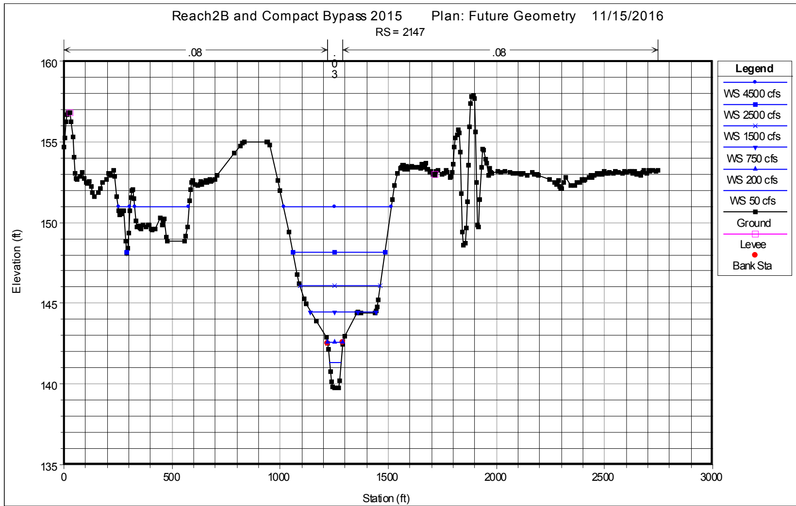
Figure 5-7.—Cross Section 2147 in Bypass showing water surfaces.
