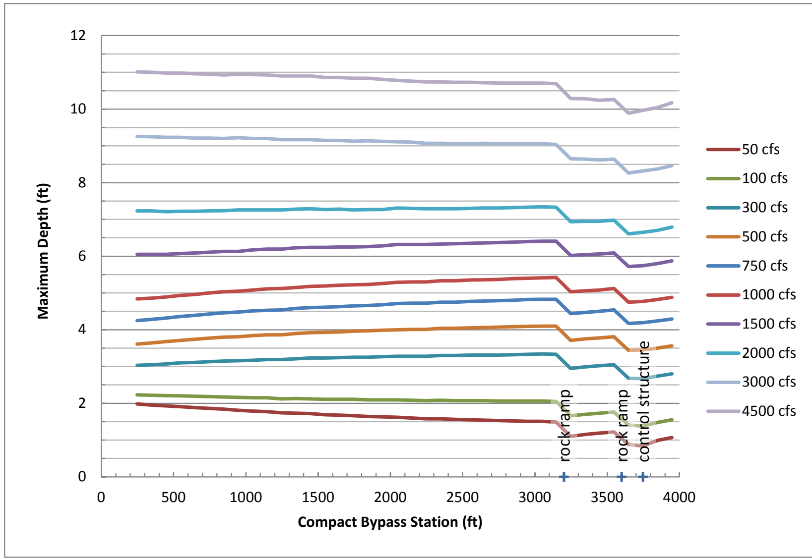
Figure 5-10.—Channel depth in Bypass for flows between 50 and 4,500 cfs.
