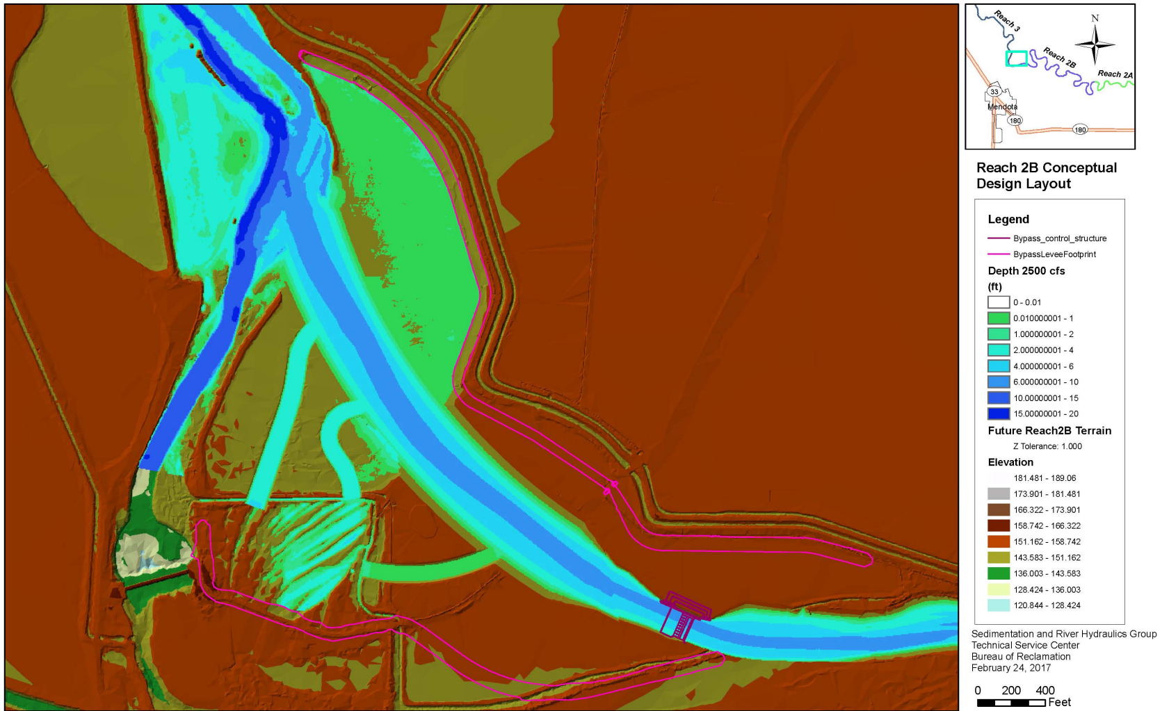
Figure 5-13.—Simulated depth distribution in the Bypass using SRH-2D at a flow of 2,500 cfs in Bypass.
