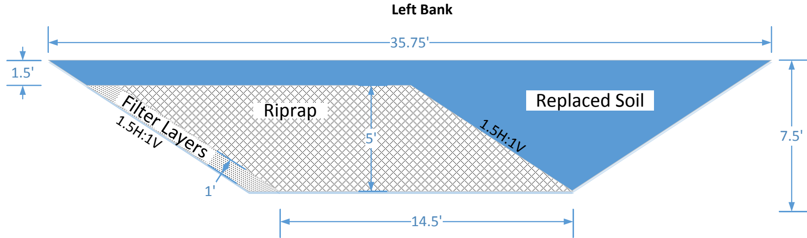
Figure 4-8.—Conceptual cross section of riprap filled trench.
