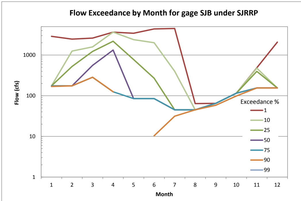
Figure 2-5.—Simulated monthly average flow rate at SJB (stream gage at upstream end of Reach 2B) under the SJRRP. The 99 percent exceedance is 0 for all months and not shown on log-scale plot.
