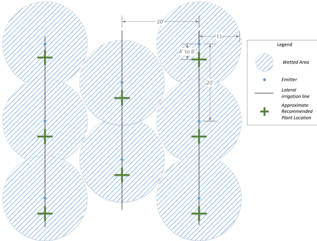
Figure 4-17.— Irrigation and Emitter spacing for Upland Woody Irrigation Zone.
