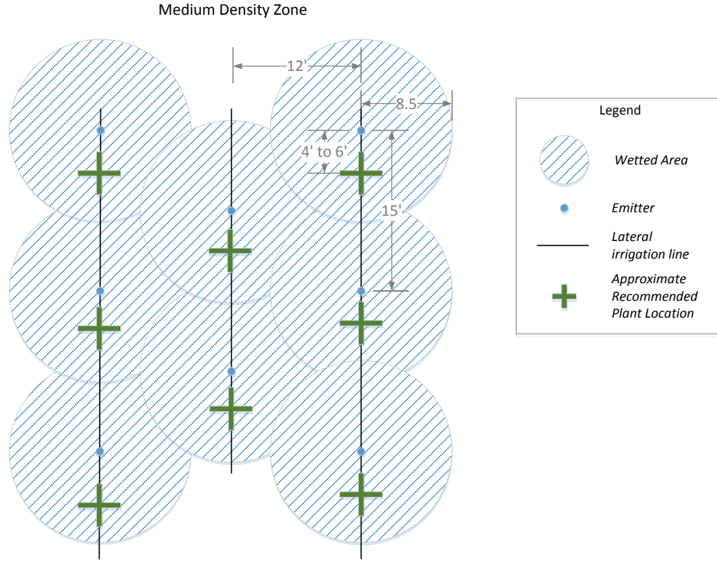
Figure 4-15.— Irrigation and Emitter spacing for Medium Density Irrigation Zone.
