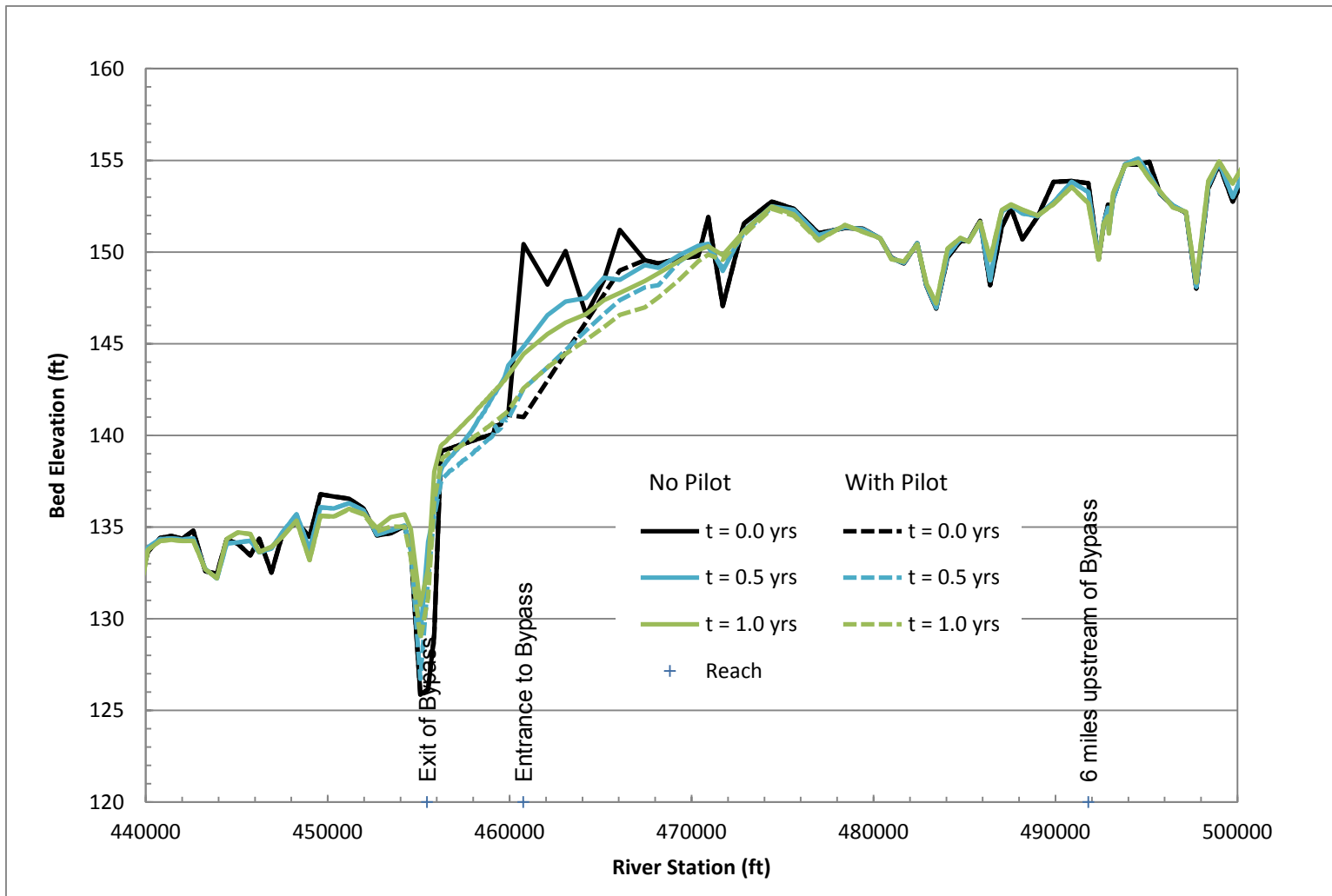
Figure 5-25.—Comparison of bed elevation with and without pilot channel for initial conditions, 0.5 years, and 1.0 years after beginning simulation.
