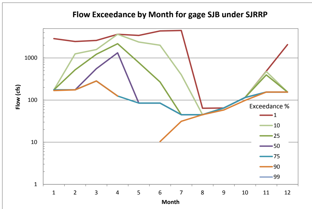
Figure 5-1.— Flow Exceedance by Month for gage SJB (in Reach 2B) under the SJRRP.
