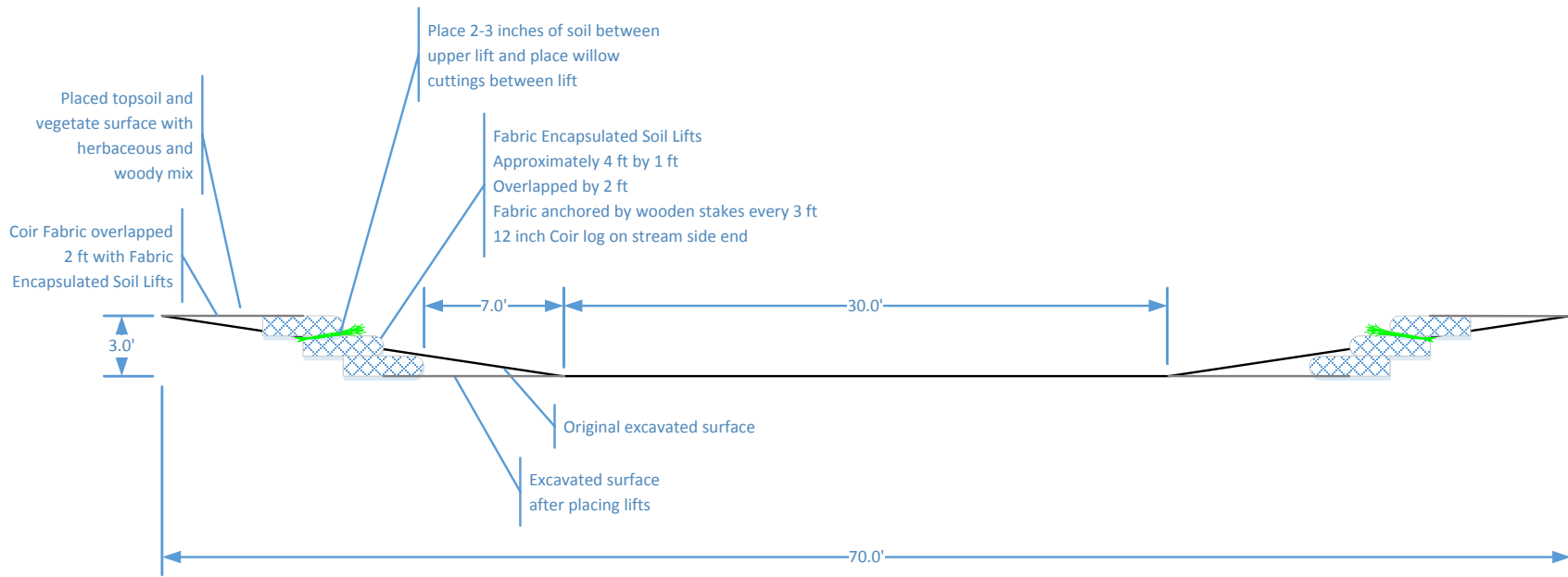
Figure 4-10.— Conceptual cross section showing placement of FES and low flow scour protection.
