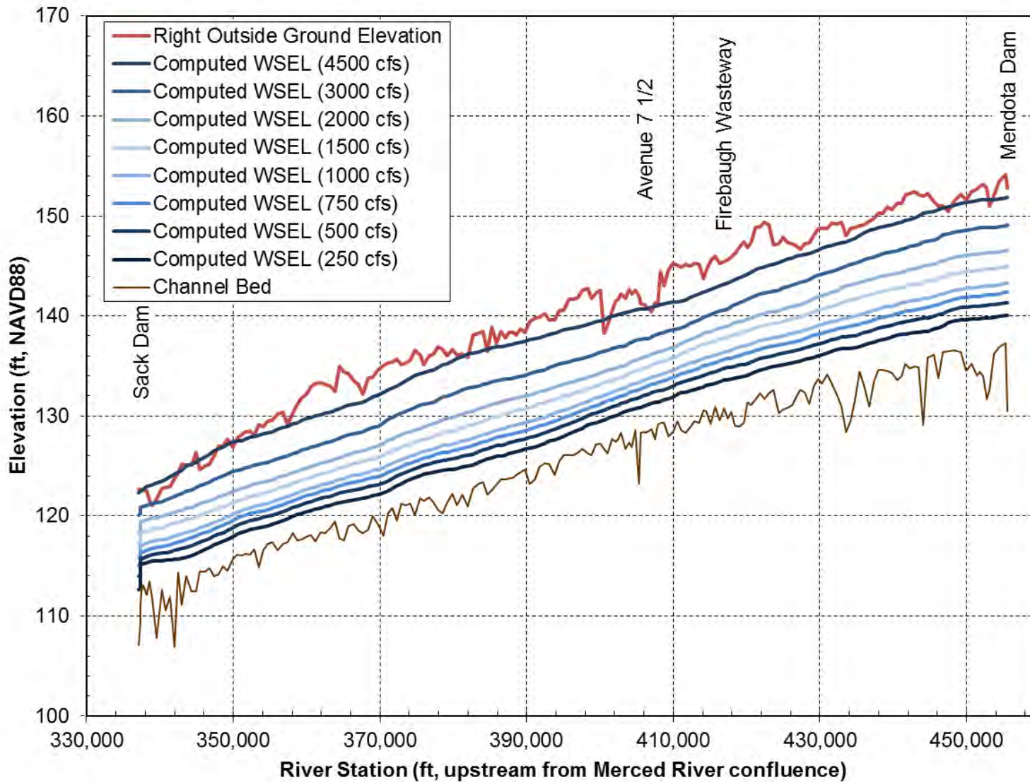
Figure 11. Comparison of outside ground elevation with computed water-surface elevations along right levee in Reach 3.
