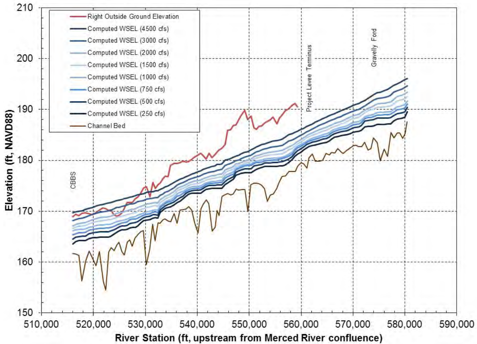
Figure 3. Comparison of outside ground profile with computed water-surface elevations along right levee in Reach 2A.
