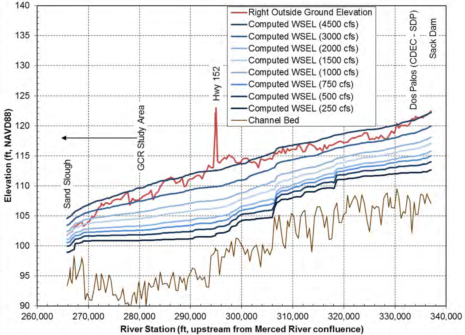
Figure 14. Comparison of outside ground elevation with computed water-surface elevations along right levee in Reach 4A.
