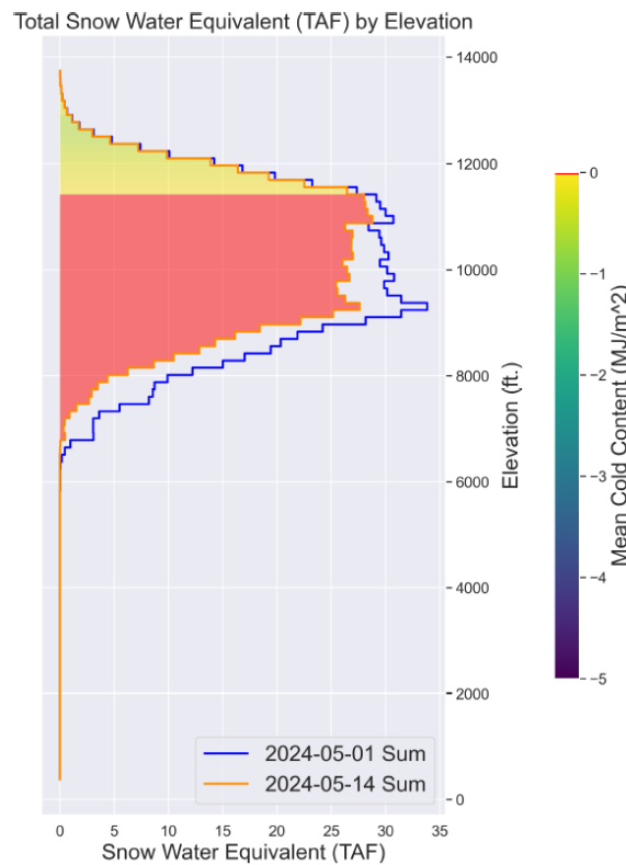
Figure 4 — iSnoPal model state on May 14 showing SWE volume by elevation and cold content. This graph depicts snowmelt from May 1 (the date of the previous ASO survey) to May 14. The color depicts the mean cold content of the snow, with all elevations below 11,500' having “ripe” conditions and more prone to melt. This is a physical distributed model produced by M3Works through a partnership with ASO Inc.
