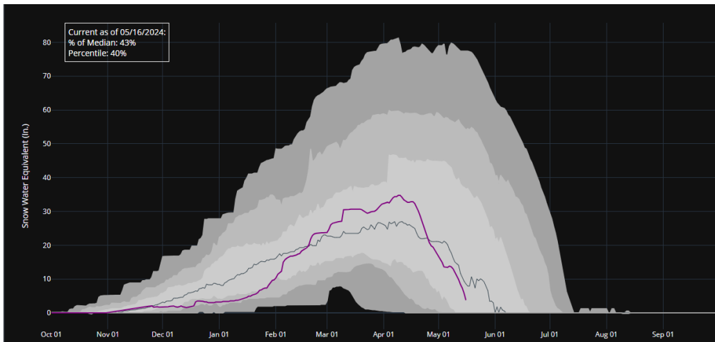
Figure 3 — Kaiser Point Snow Pillow trace. The rate of melt at this snow pillow at 9200' elevation (purple line) has exceeded the median trace (gray line), indicative of rapid melt.
