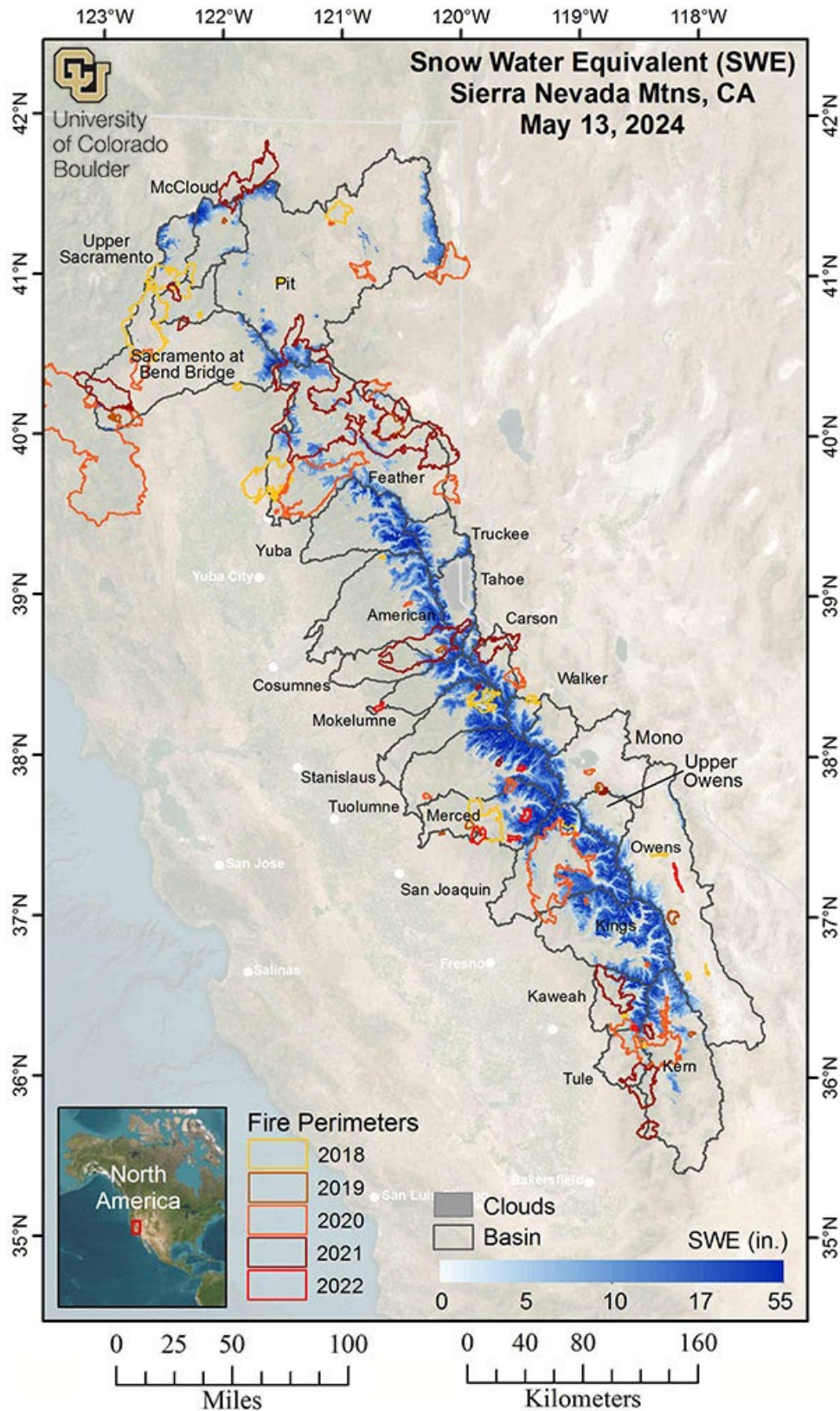
Figure 5 — Sierra Nevada snowpack as modeled by University of Colorado Boulder’s “Real-time SWE” model on May 13. This is a fusion model which combines snow-covered area estimates from satellite, ground-based stations, and statistical relationships. The 2020 “Creek Fire” burn area is shown within the Upper San Joaquin watershed. The snowline has now retreated to higher elevations above the burned area.
