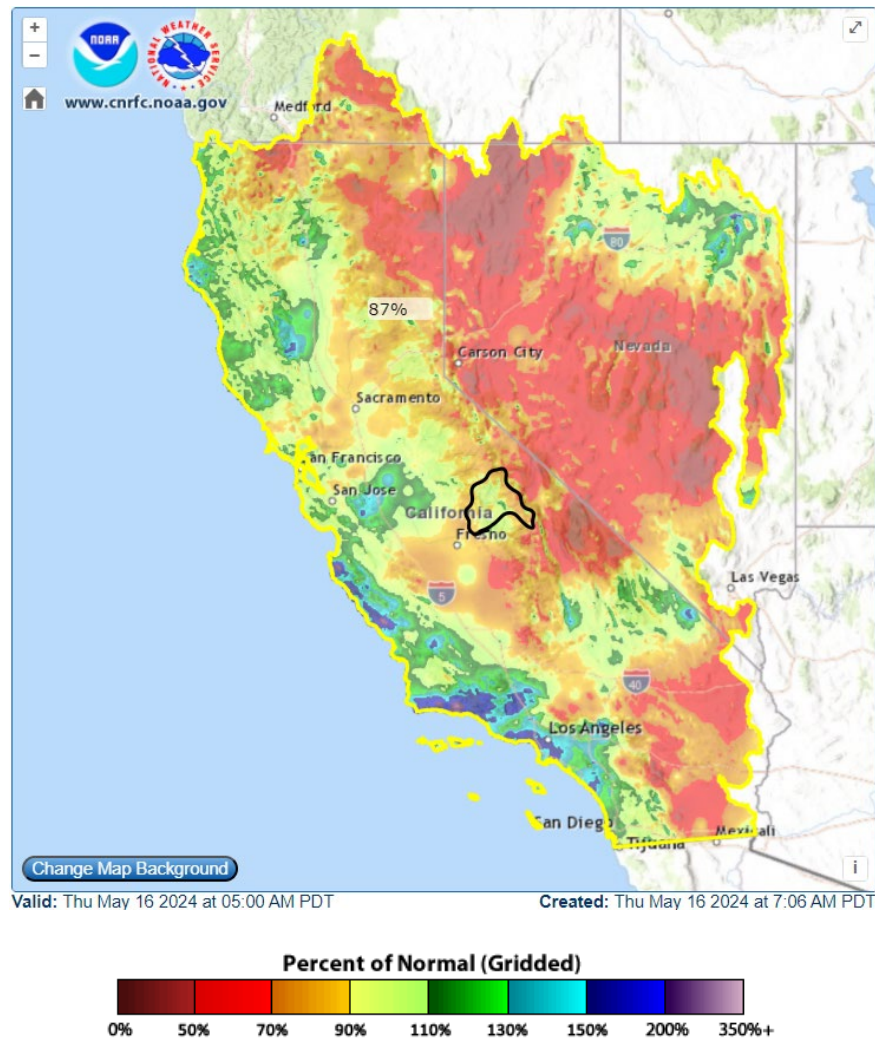
Figure 2 — California Water Year Precipitation as a percent of average. The Sierra Nevada has received near-normal precipitation, with somewhat lower amounts in the Southern Sierra. The Upper San Joaquin watershed is outlined.
