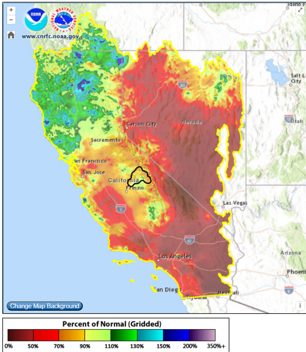
Figure 2. California Water Year Precipitation as a percent of average. A strong gradient from north to south developed early in the water year, however February and early March storms have evened out the differences from north to south.
