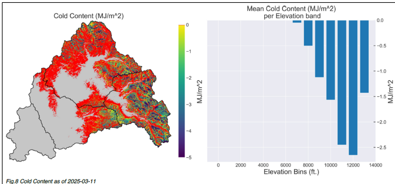
Figure 5. Modeled snowpack cold content. Cold content is driven by the temperature of the storms which deposited the snow, the intervening weather between storms, and the snowpack albedo. Warmer storms and impurities in the snowpack at lower elevations have resulted in very low cold content below 9,000 feet
