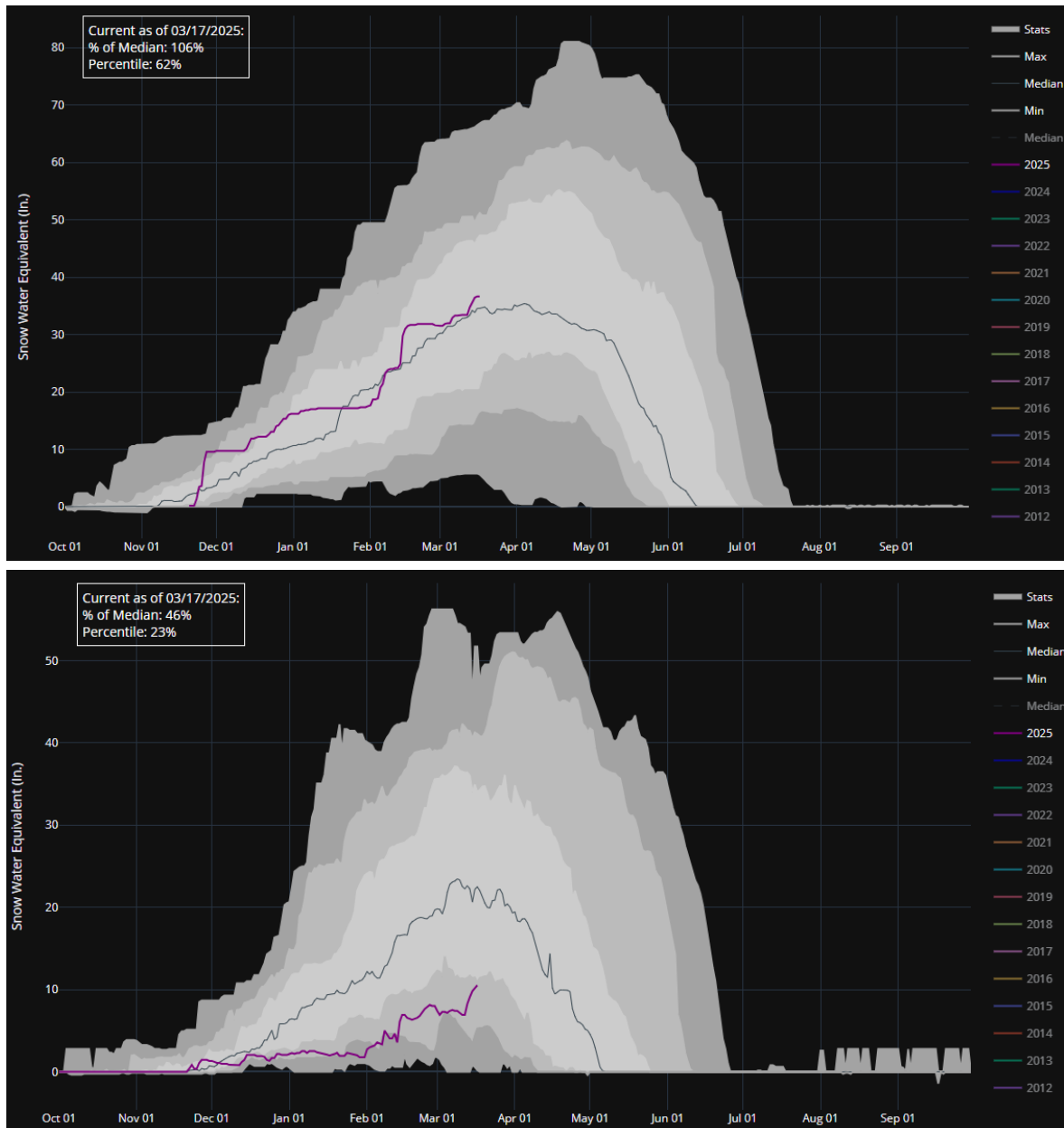
Figure 3. Mammoth Pass Snow Pillow trace (top) compared to Poison Ridge Snow Pillow trace (bottom). Snow Water Equivalent (SWE) is plotted here as purple line against historic probabilities at two of the many snow pillows. Mammoth Pass SWE is tracking near-median conditions and lies at 9,300 feet elevation, whereas Poison Ridge SWE is well below median conditions and lies at 6,900 feet elevation.
