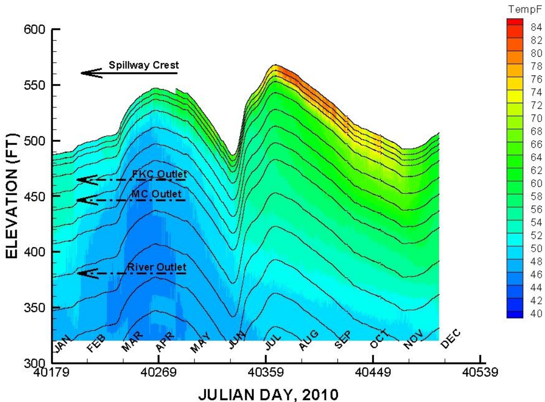
Figure 2-3. 2010 Friant Dam Forebay Temperature Profiles
