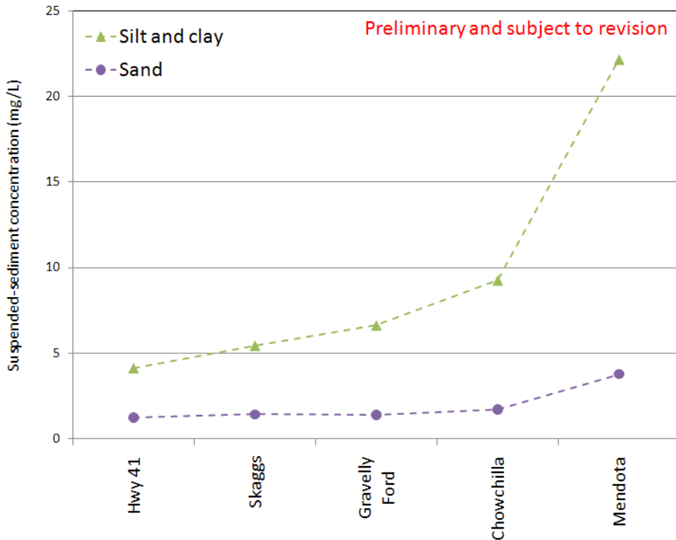
8 Figure 2-8. Averaged Suspended Sediment Concentrations
