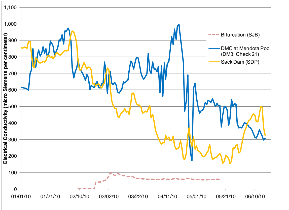
1 Figure 2-6. Electrical Conductivity of Surface Water at the Chowchilla Bifurcation 2 station, Sack Dam, and the Delta Mendota Canal at Mendota Pool
