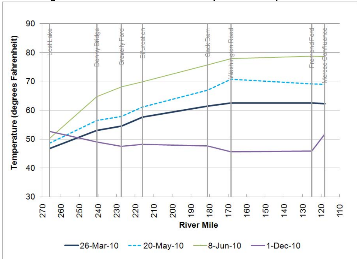
12 Figure 2-4. 2010 Interim Flows San Joaquin River Temperatures
