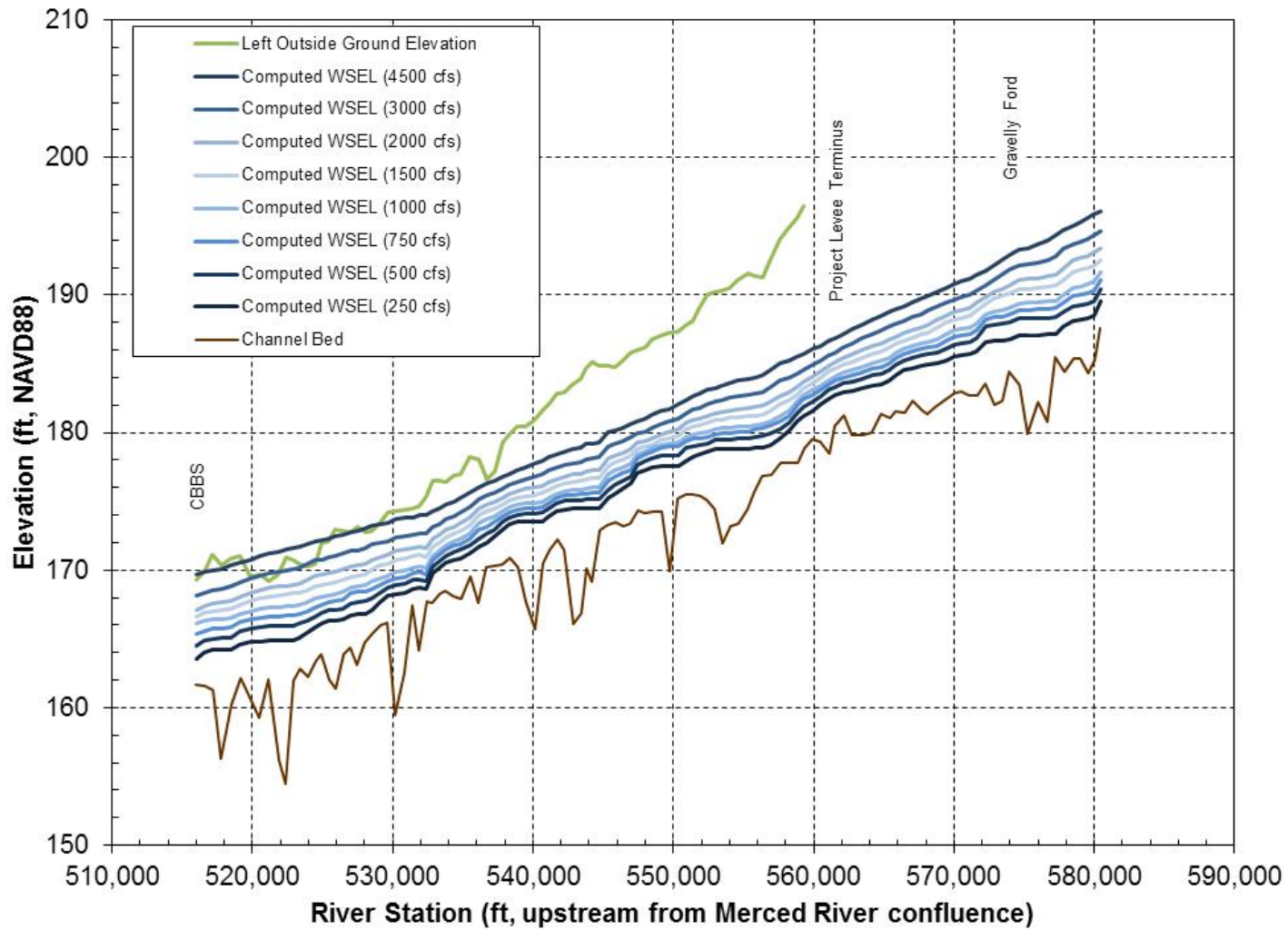
Figure 3. Comparison of outside ground profile with computed water-surface elevations along left levee in Reach 2A.
