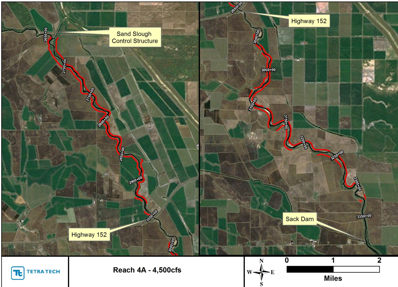
Figure 16. Portions of levee in Reach 4A where the 4,500-cfs water-surface elevation is above the existing outside ground elevation.
