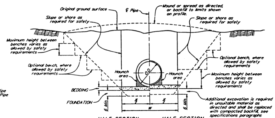
HALF SECTION RIGID PIPE HALF SECTION FLEXIBLE PIPE TYPICAL TRENCH DETAILS
