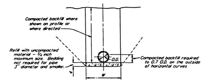
PIPE 10 INCH DIAMETER AND SMALLER
