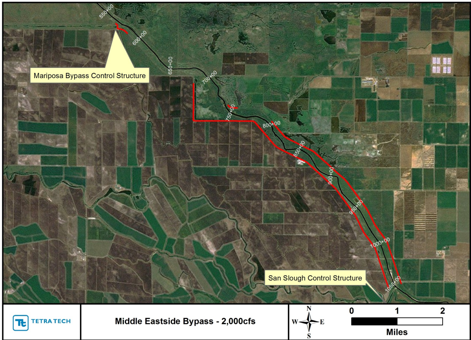
Figure 27. Portions of levee in the Middle Eastside Bypass where the 2,000-cfs water-surface elevation is above the existing outside ground elevation.
