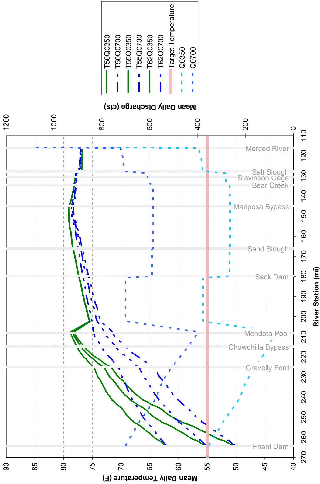
Figure B-13 Set 2 Profile of Median Mean Daily Temperature Values for the Time Period of September
