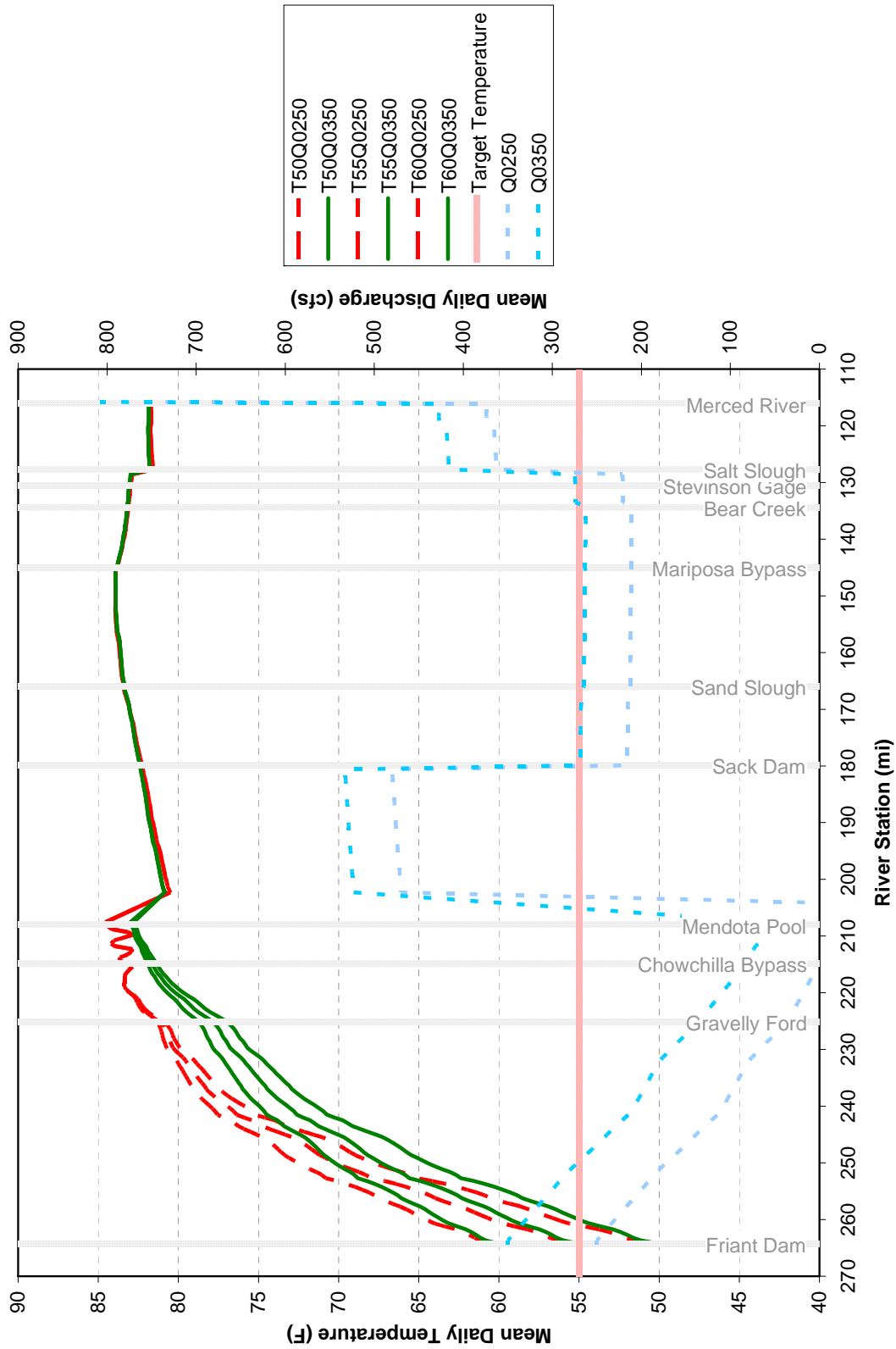
Figure B-12 Set 2 Profile of Median Mean Daily Temperature Values for the Time Period of August
