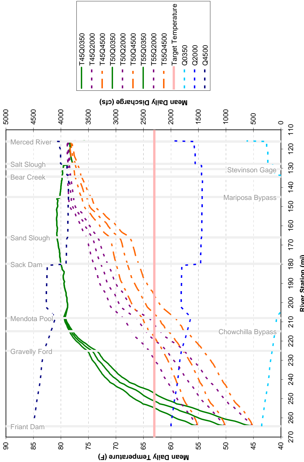
Figure B-10 Set 2 Profile of Median Mean Daily Temperature Values for the Time Period of June
