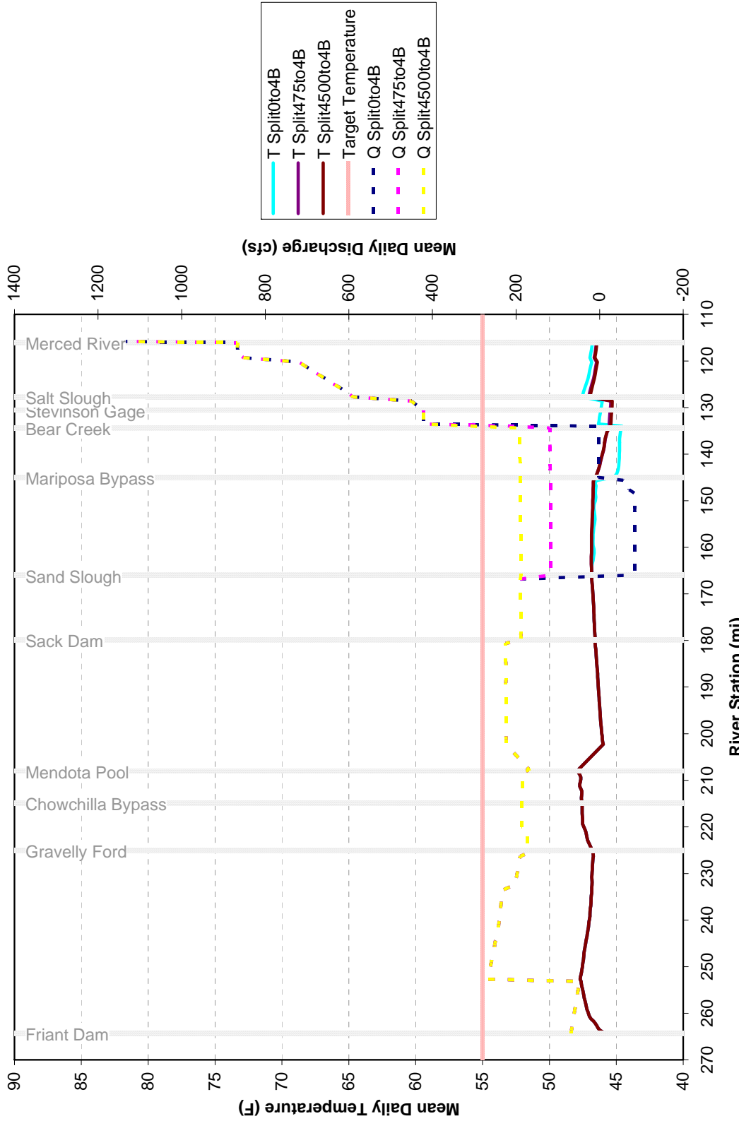
Figure A-1 Set 1 Profile of Median Mean Daily Temperature Values for the Time Period of January
