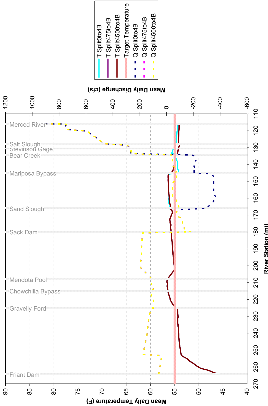
Figure A-2 Set 1 Profile of Median Mean Daily Temperature Values for the Time Period of February
