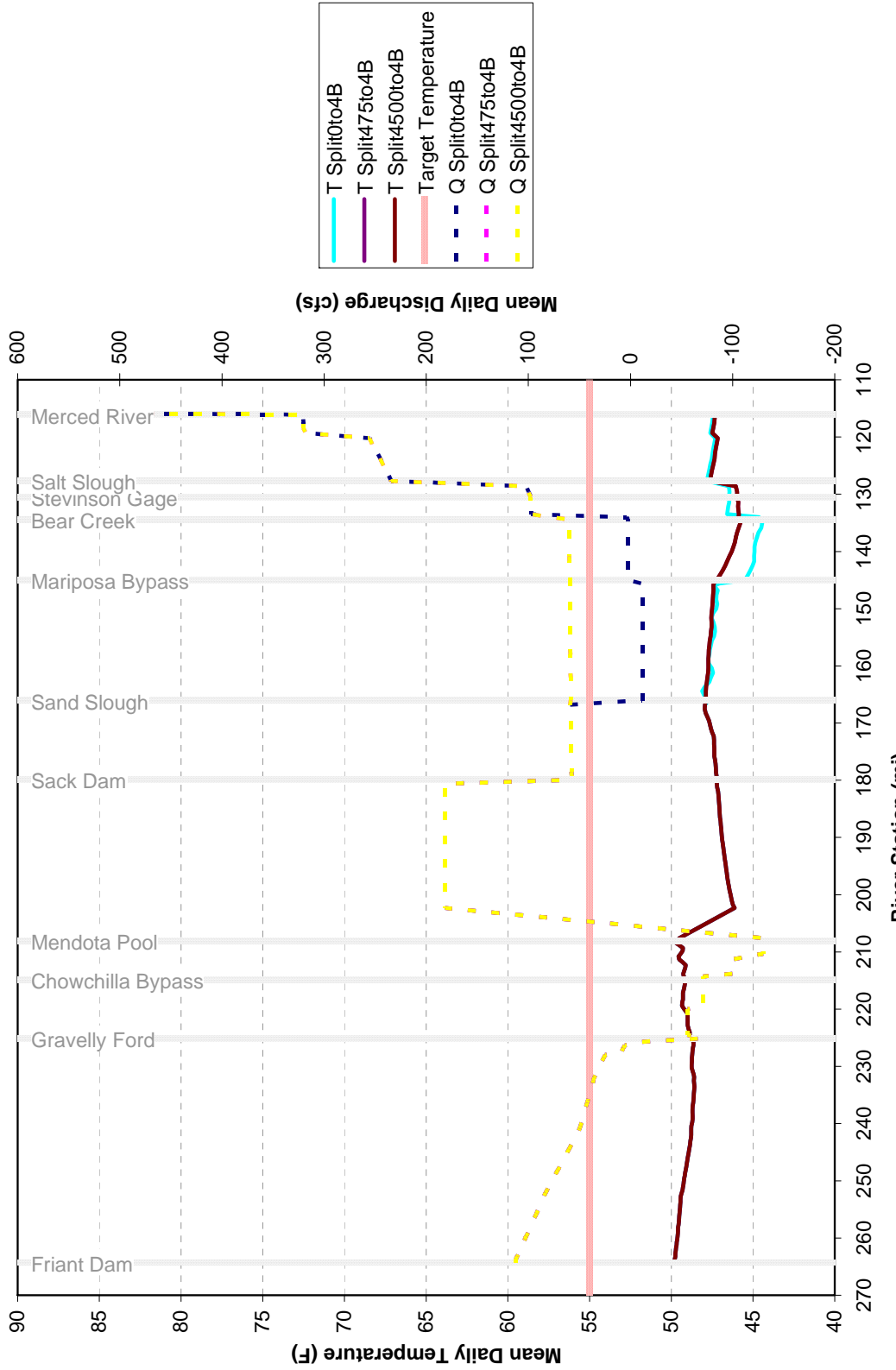
Figure A-26 Set 1 Profile of Median Mean Daily Temperature Values for the Time Period of December
