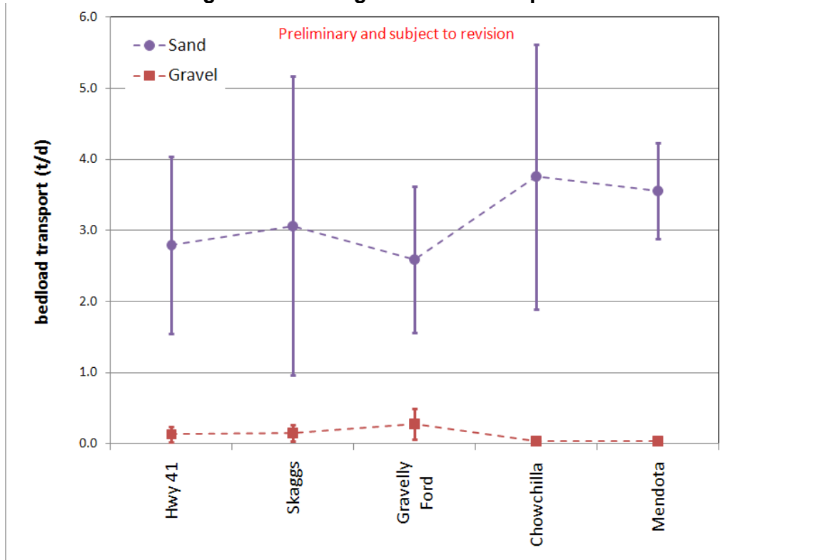
Figure 2-9. Average Bedload Transport Rates 1
